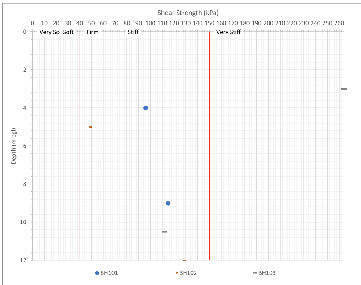
Figure 5: Shear Strength Test Results
