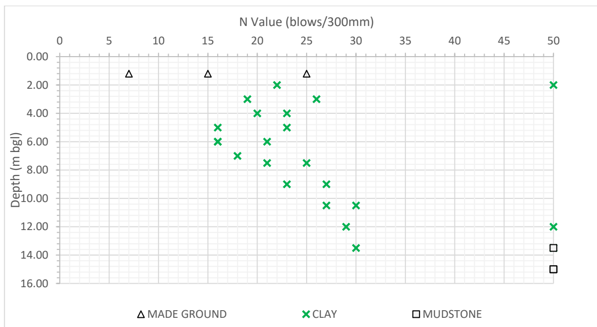
Figure 3: SPT Results
