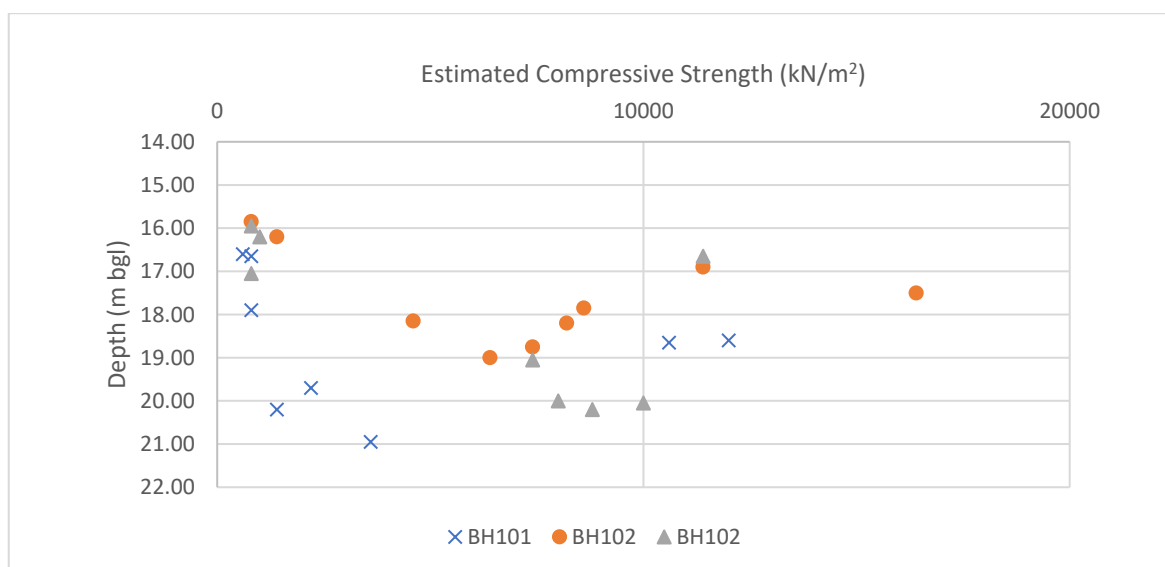
Figure 6: Point Load Results
