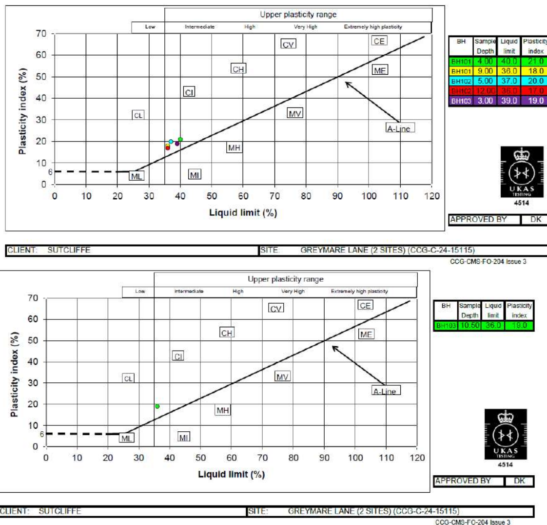
Figure 4: Plasticity Test Results
