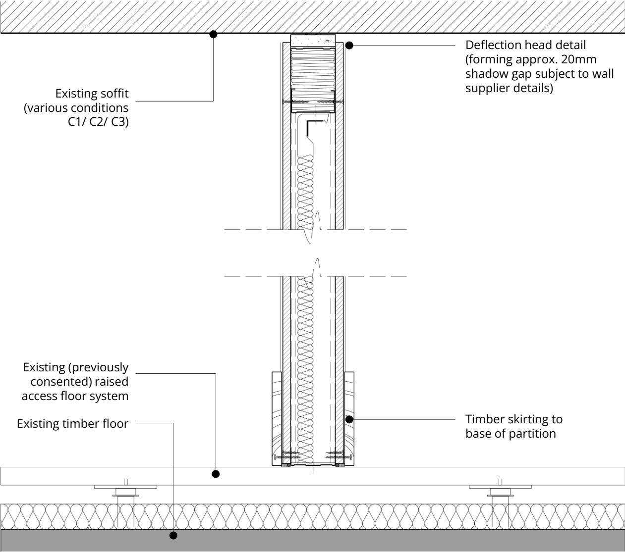
Section detail of proposed partition abutment to contemporary raised access floor and various existing/ previously consented soffit conditions (C1/ C2/ C3)
