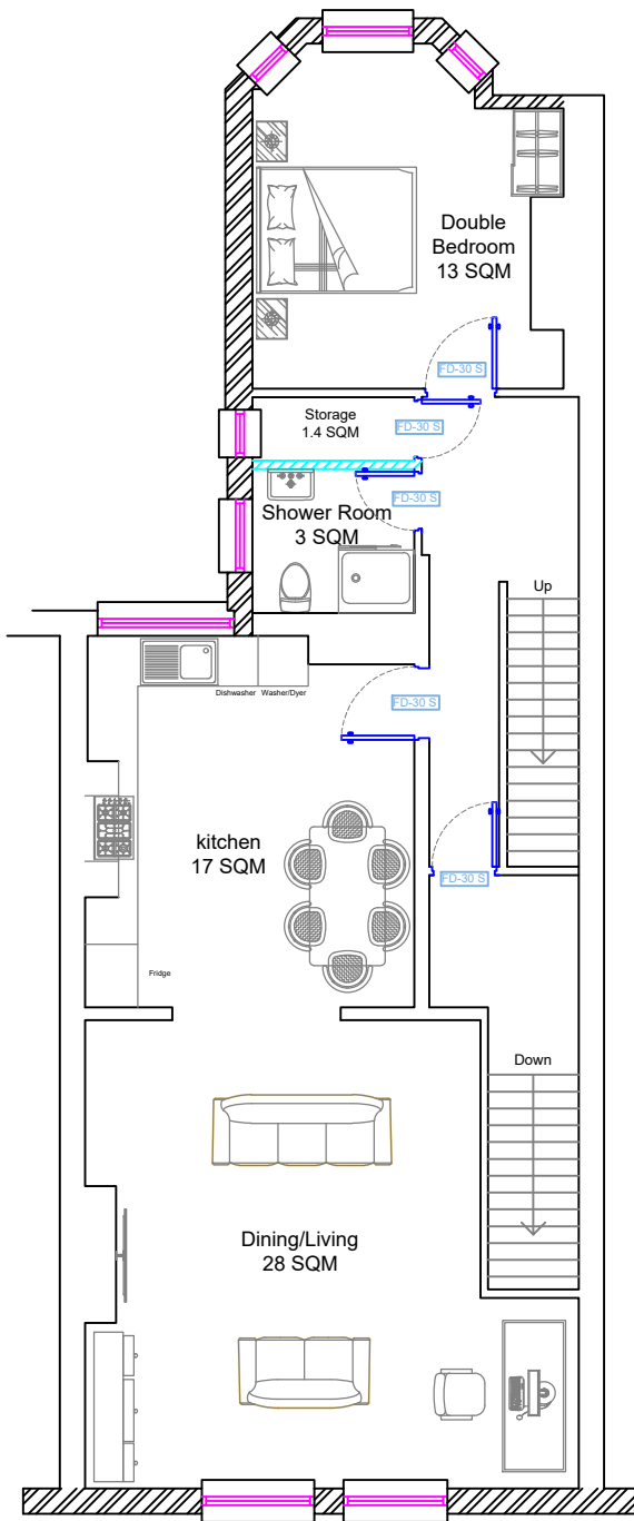
First Floor
