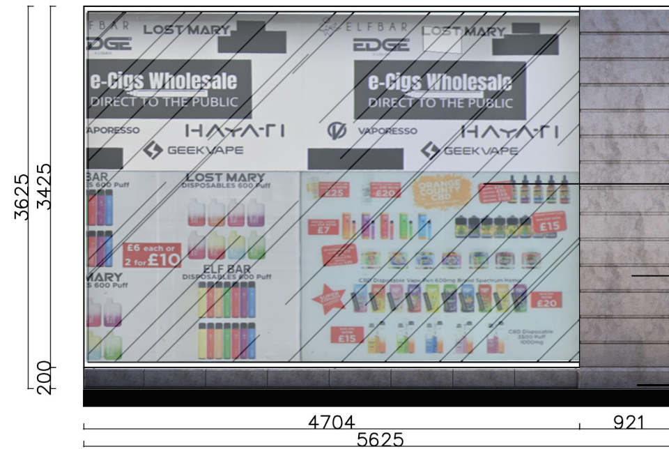
LEFT SHOPFRONT- EXISTING ELEVATION
