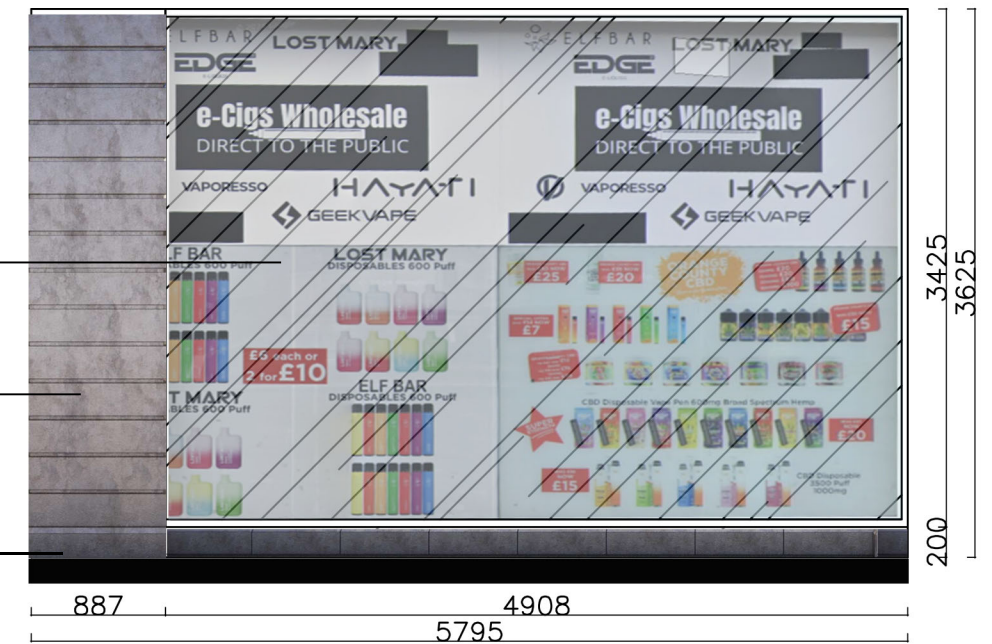
RIGHT SHOPFRONT - EXISTING ELEVATION
