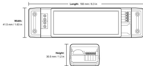
ECodrive 240/A-BIS
