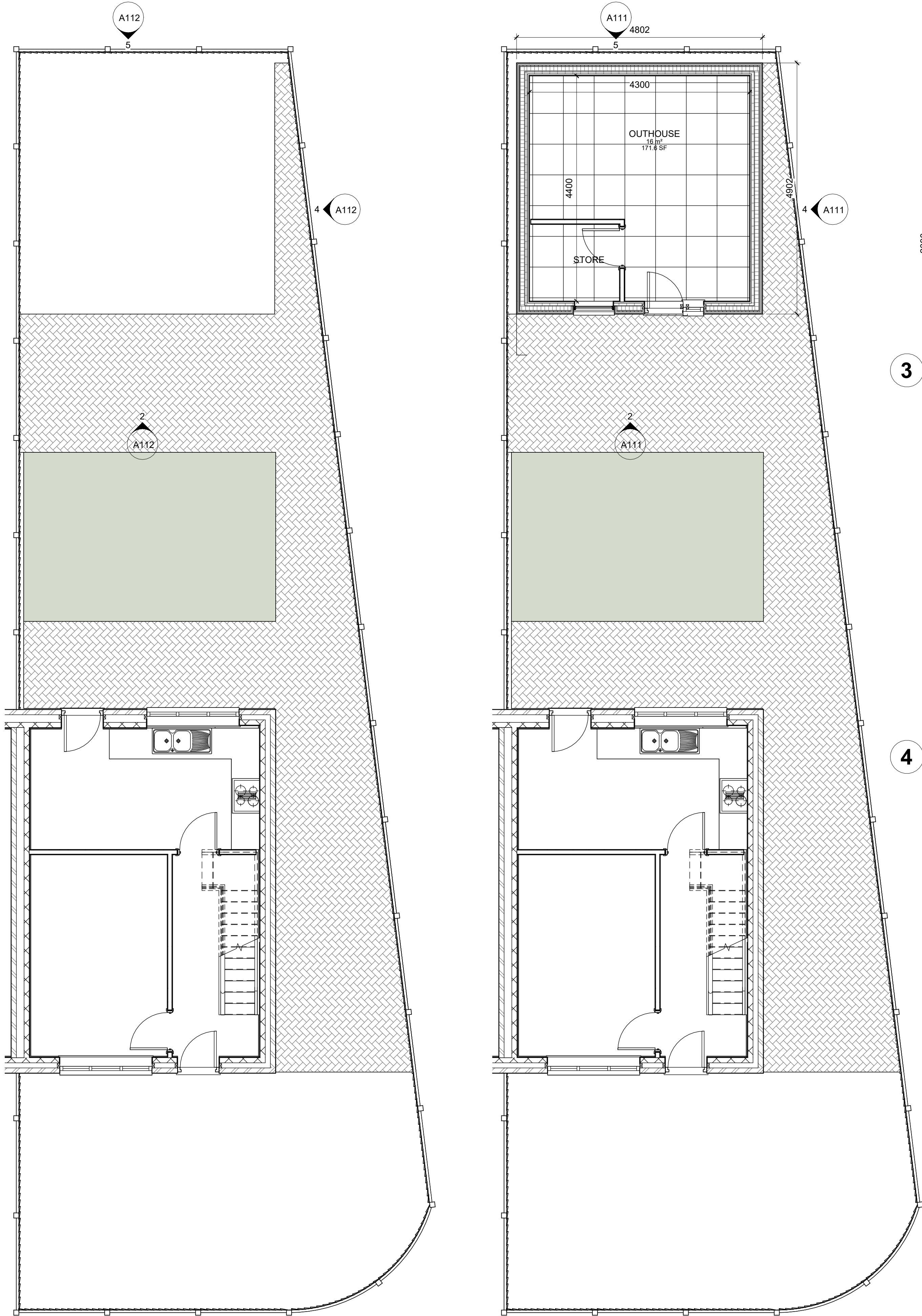
7 GF EXISTING OUTHOUSE 1 : 50
