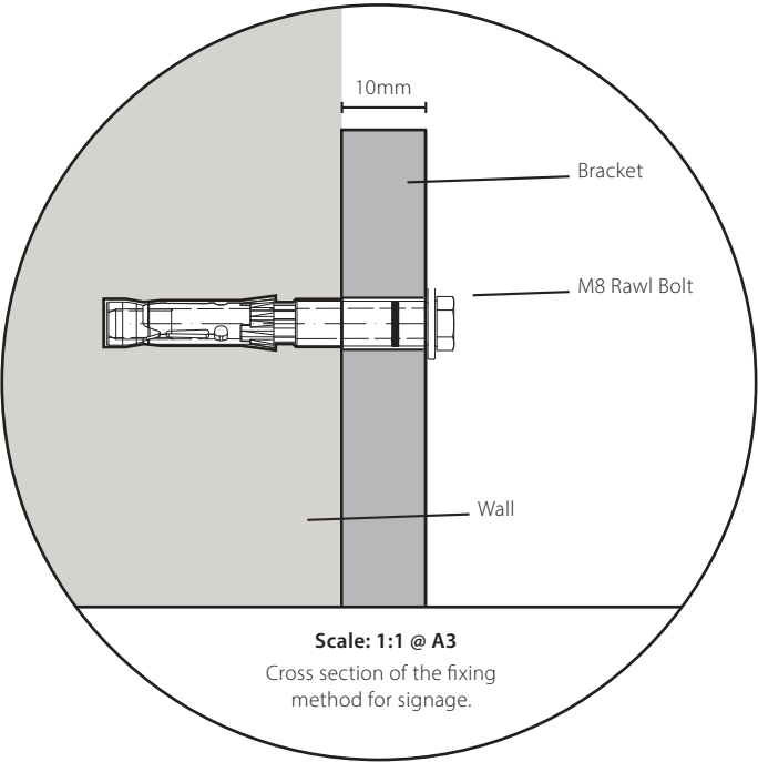
Method of fixing for Item A. (see CSI 211 A).
