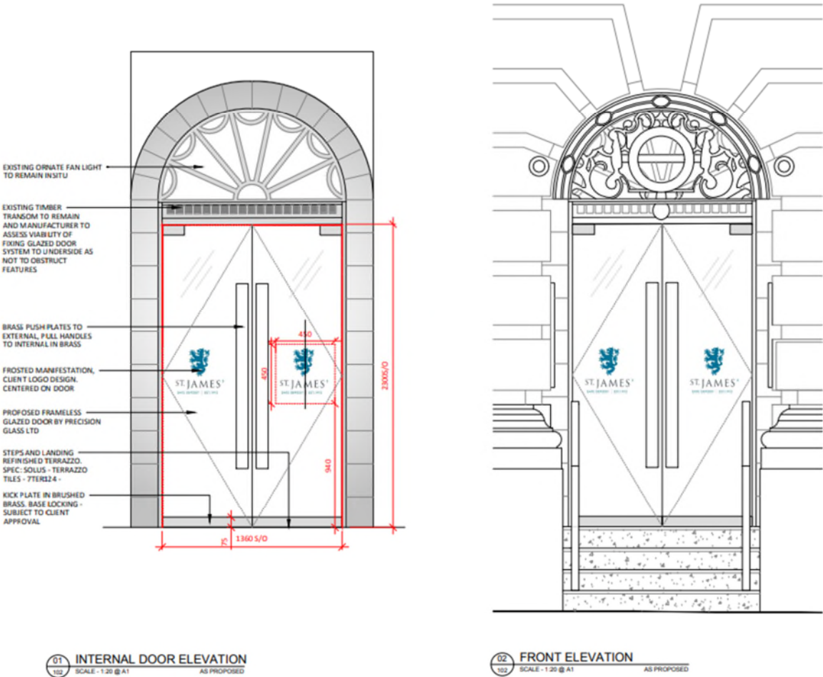
Proposed elevations
