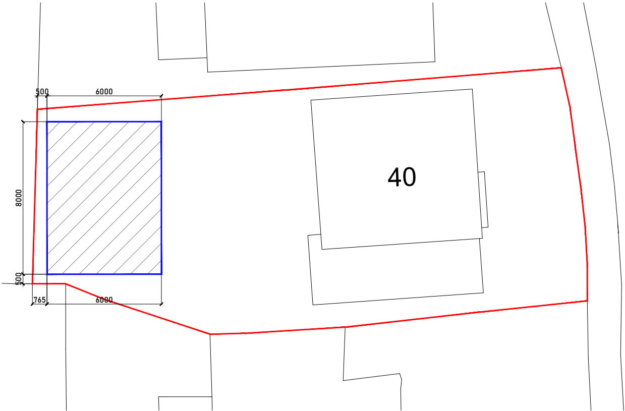
PROPOSED BLOCK PLAN 1:200
