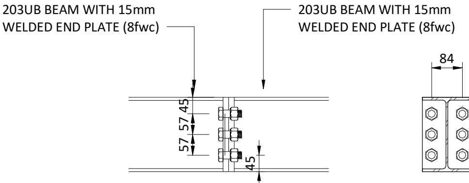
203UB SPLICE DETAIL SCALE 1 : 10
