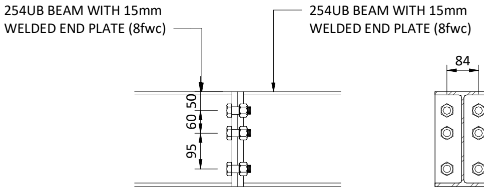
254UB SPLICE DETAIL SCALE 1 : 10
