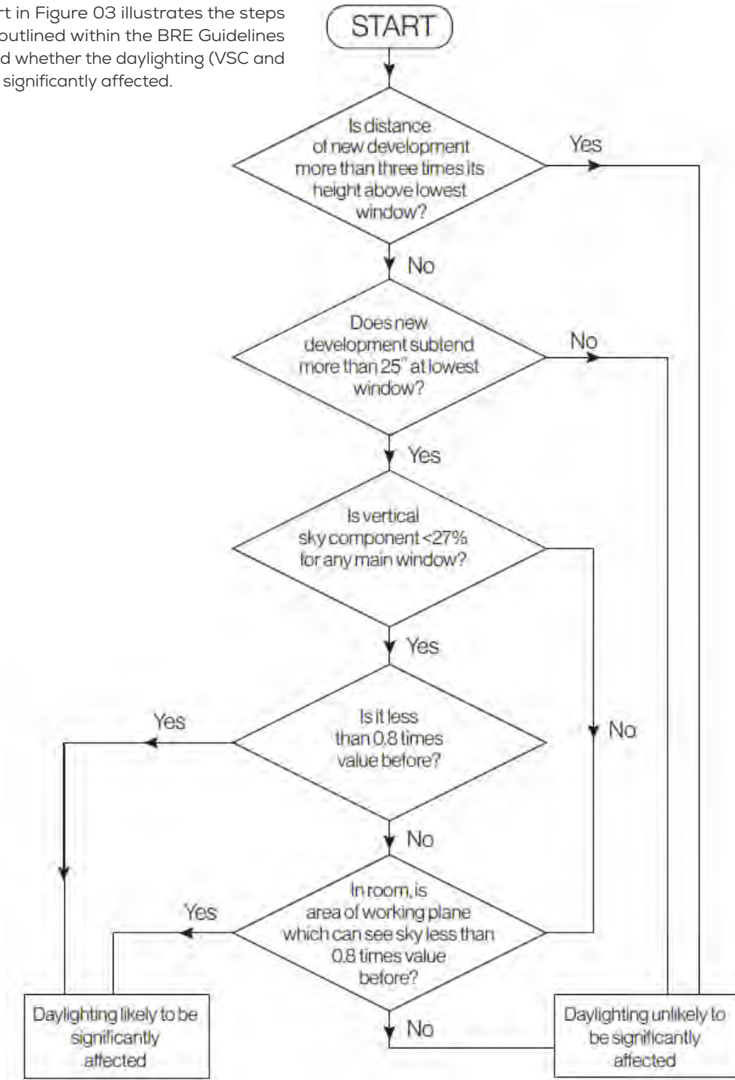
Figure 03: BRE Decision Chart (Figure 20): diffuse daylight in existing buildings. This does not include an assessment of rights to light issues, which a developer may need to consider separately
