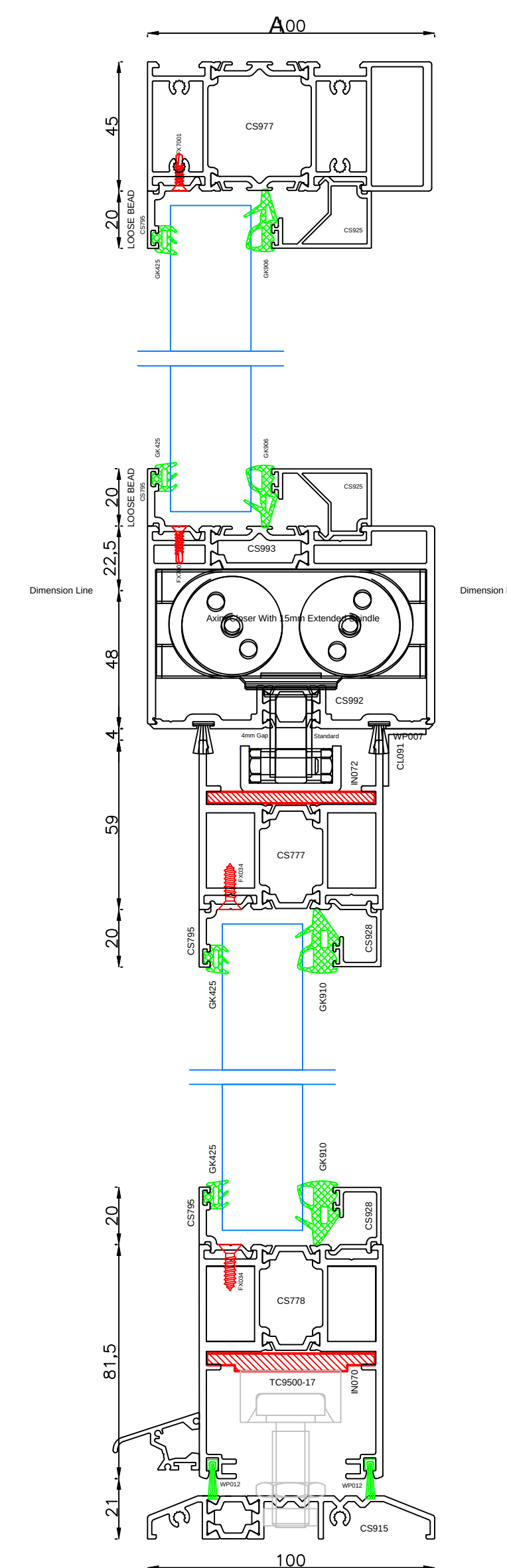
Full Height Cut Through - Cut A
