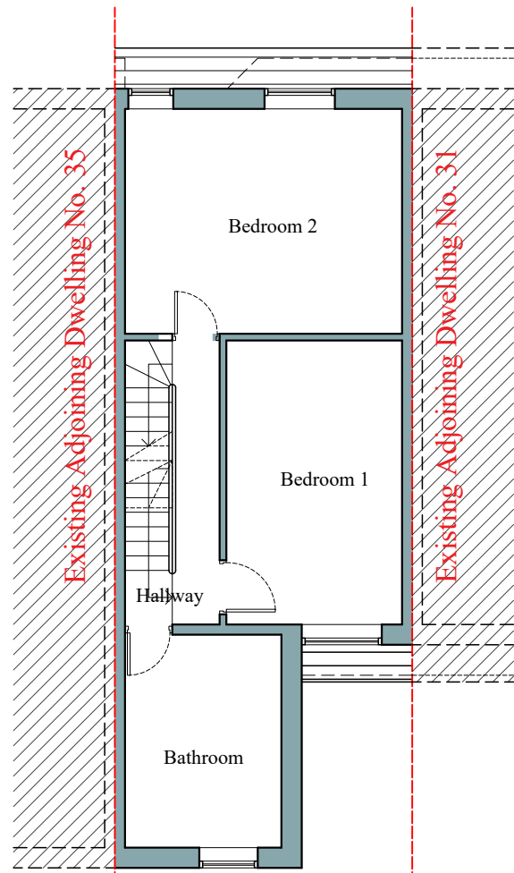
Proposed 1/F Plan 1:100
