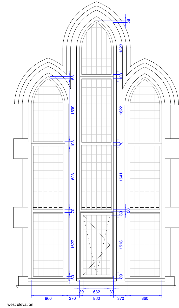
west elevation
