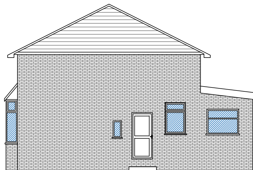
EXISTING GABLE ELEVATION
