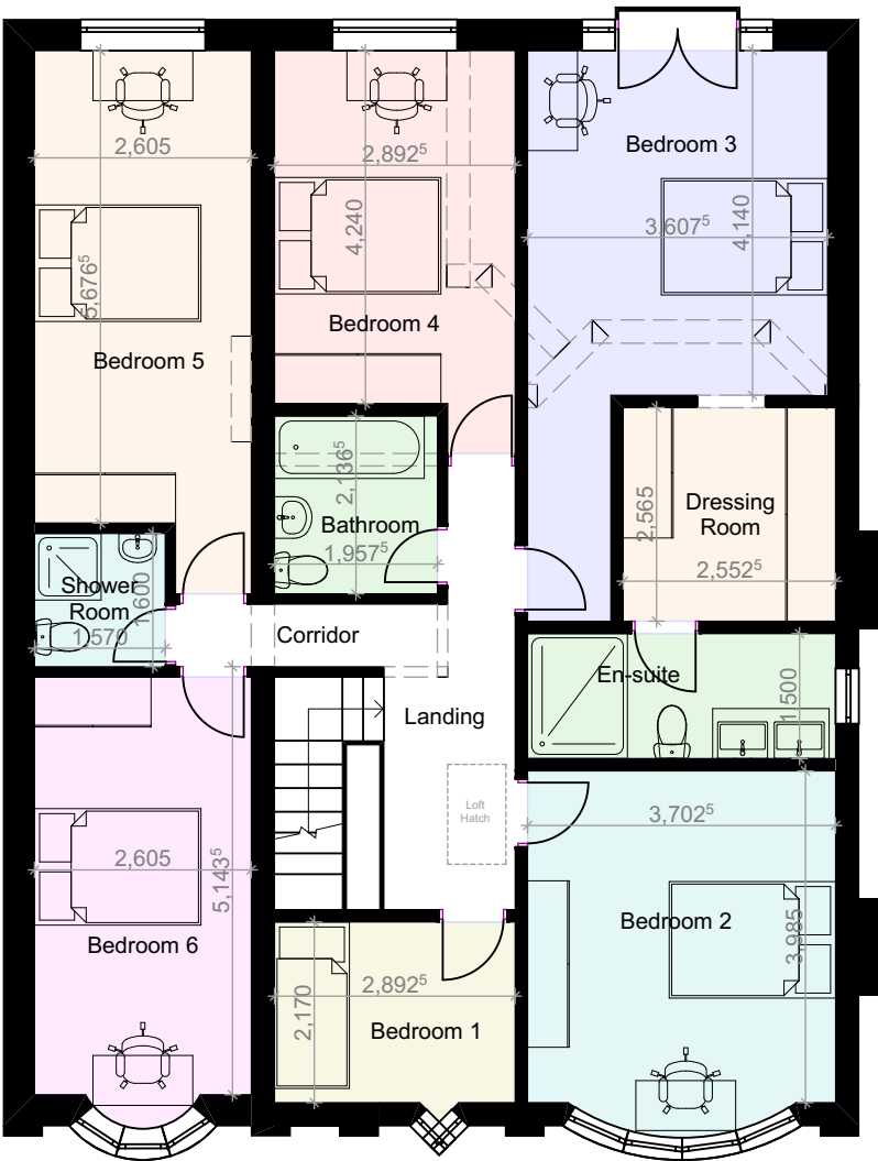
PROPOSED GA FIRST FLOOR PLAN
