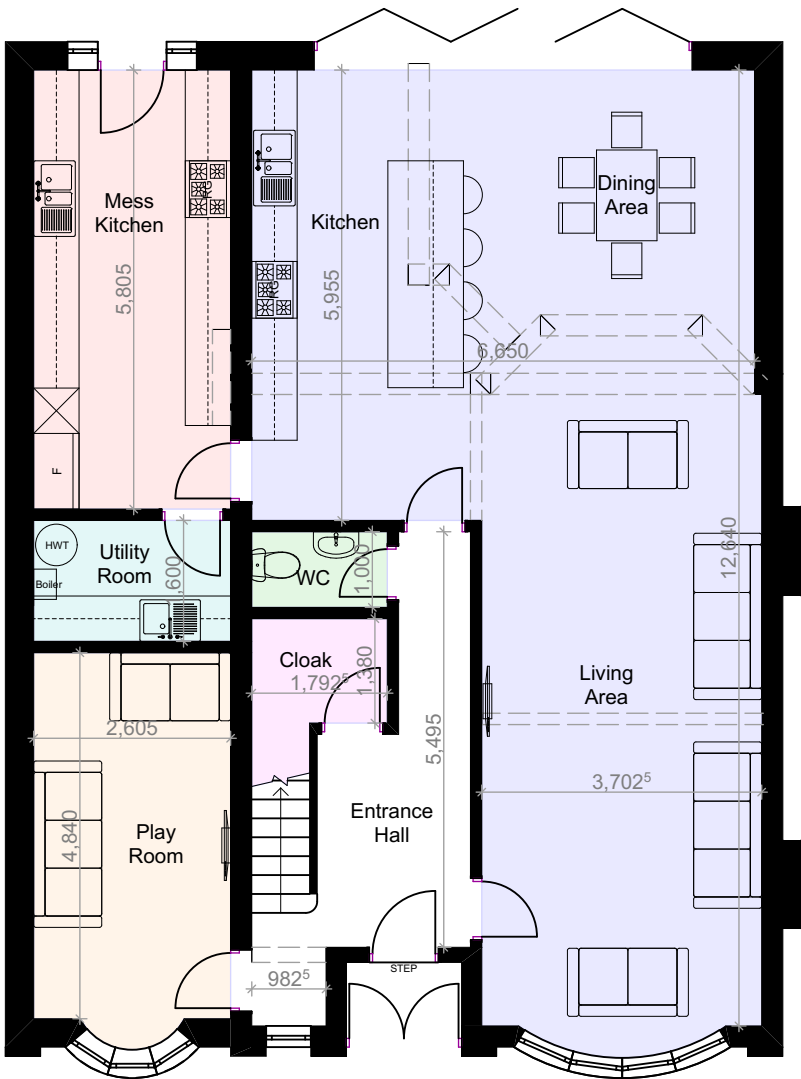
PROPOSED GA GROUND FLOOR PLAN
