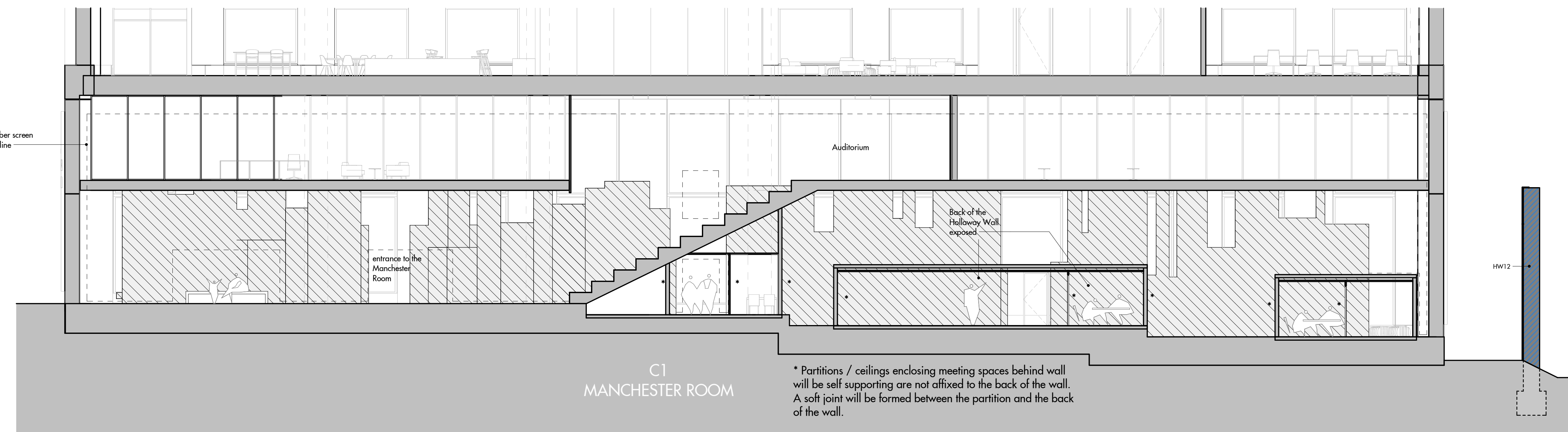
5 Holloway Wall Proposed Eastern Elevation 1 : 100
