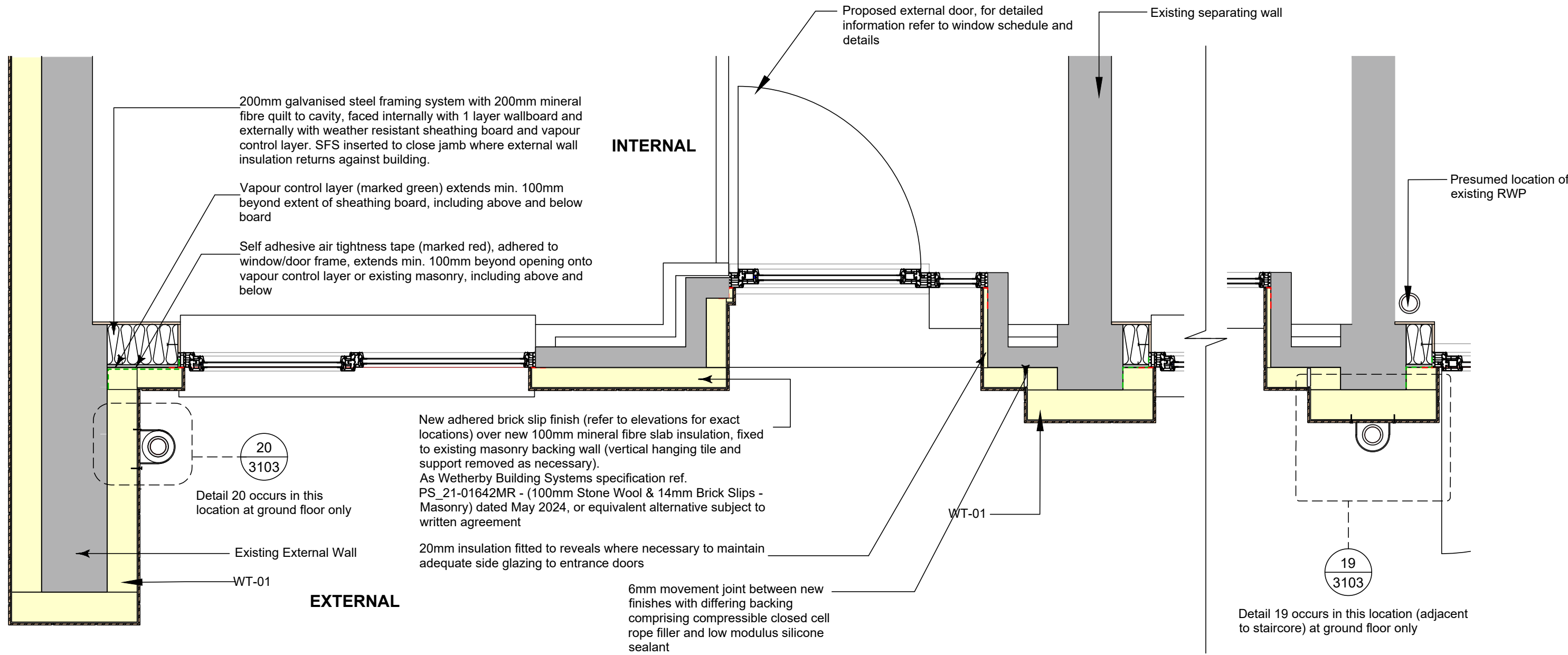
DETAIL 7 - GROUND/SECOND FLOOR MAISONETTE FRONT ENTRANCE
