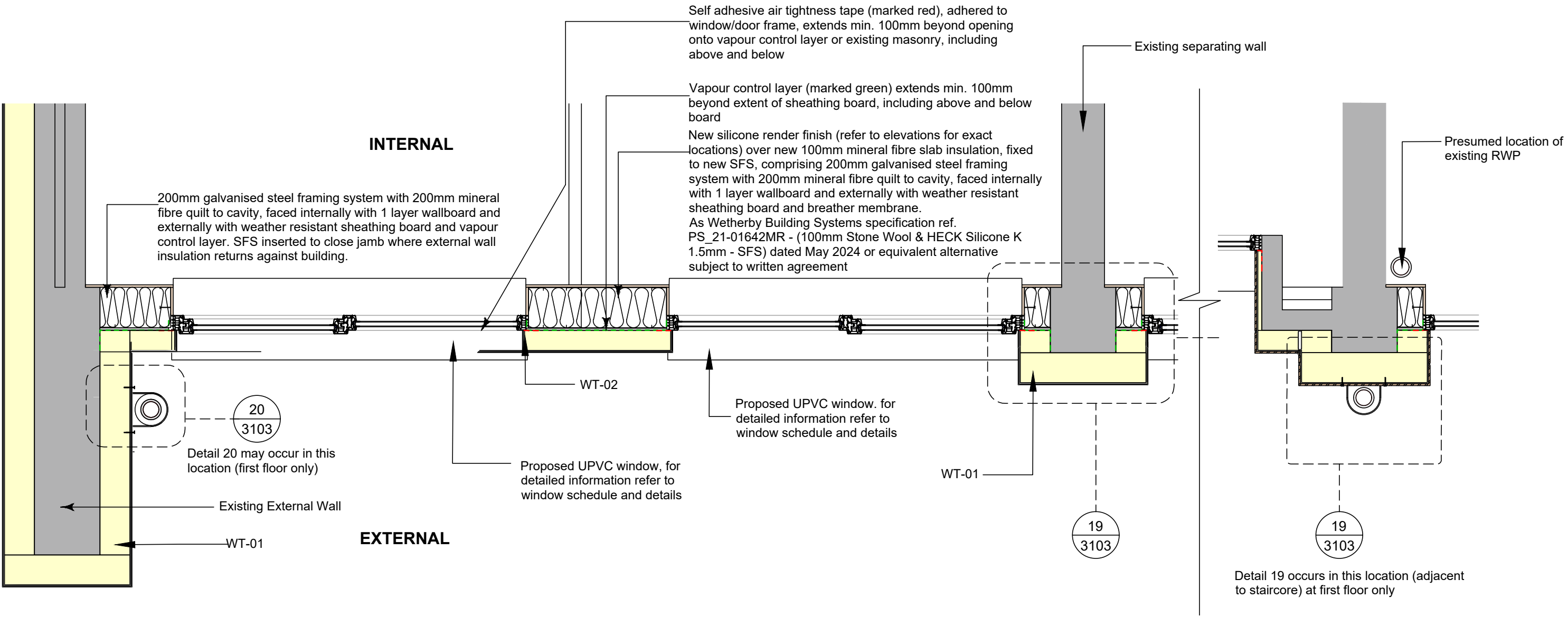
DETAIL 8 - FIRST/THIRD FLOOR MAISONETTE FRONT
