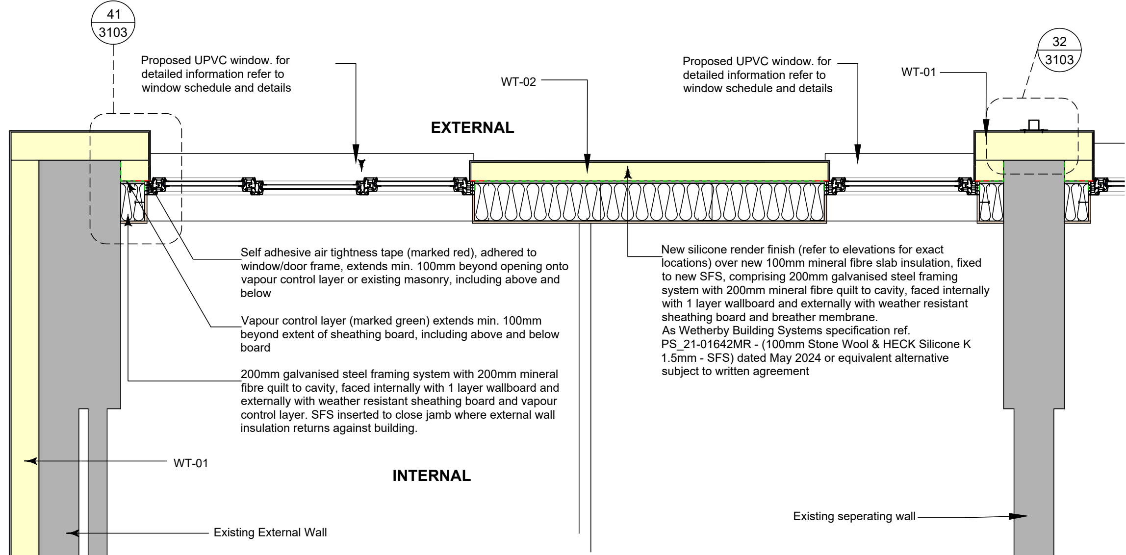
DETAIL 10 - FIRST/THIRD FLOOR MAISONETTE REAR
