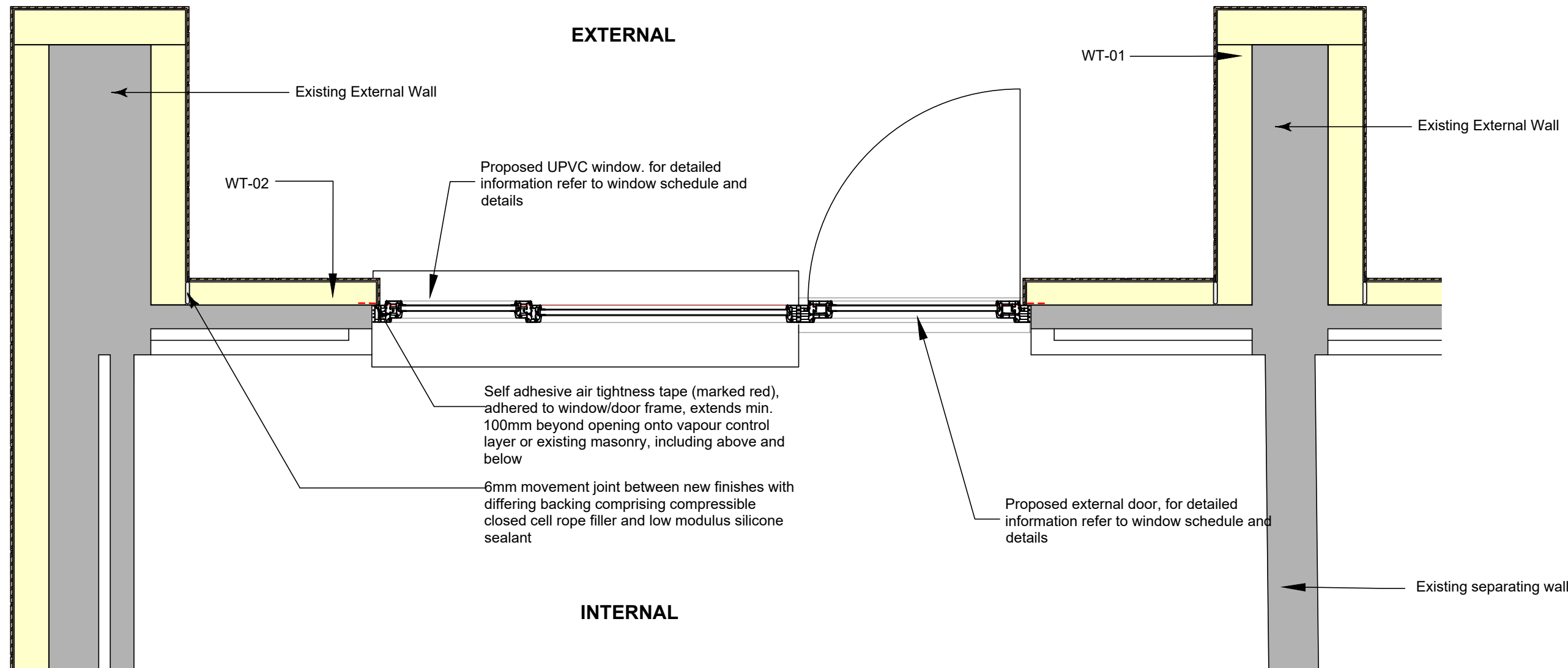
DETAIL 9 - GROUND/SECOND FLOOR MAISONETTE REAR ENTRANCE
