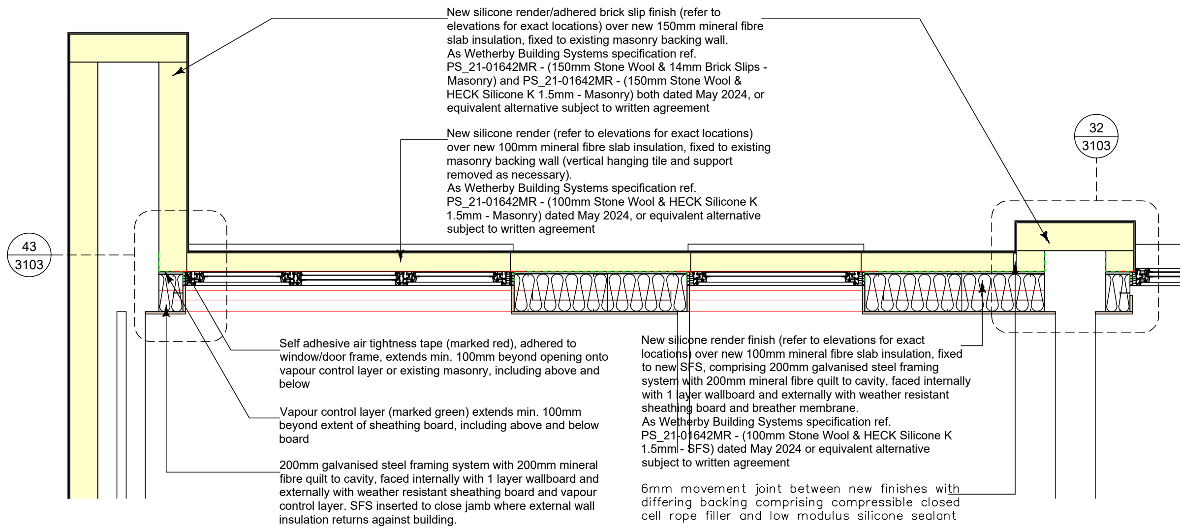
DETAIL 5 - FIRST & THIRD FLOOR MAISONETTE
