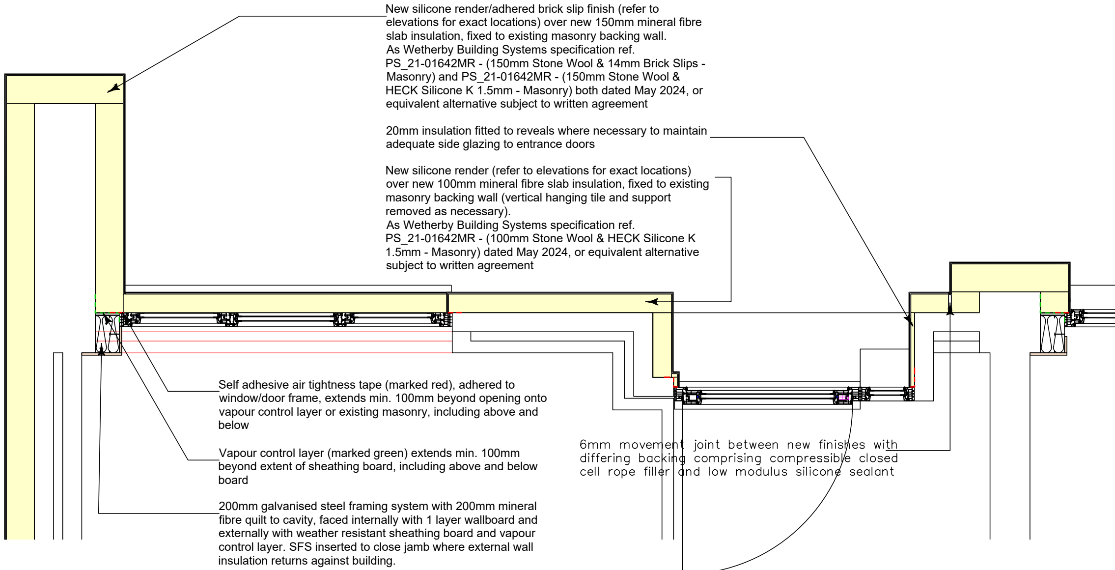
DETAIL 6 - SECOND FLOOR MAISONETTE FRONT DOOR ENTRANCE
