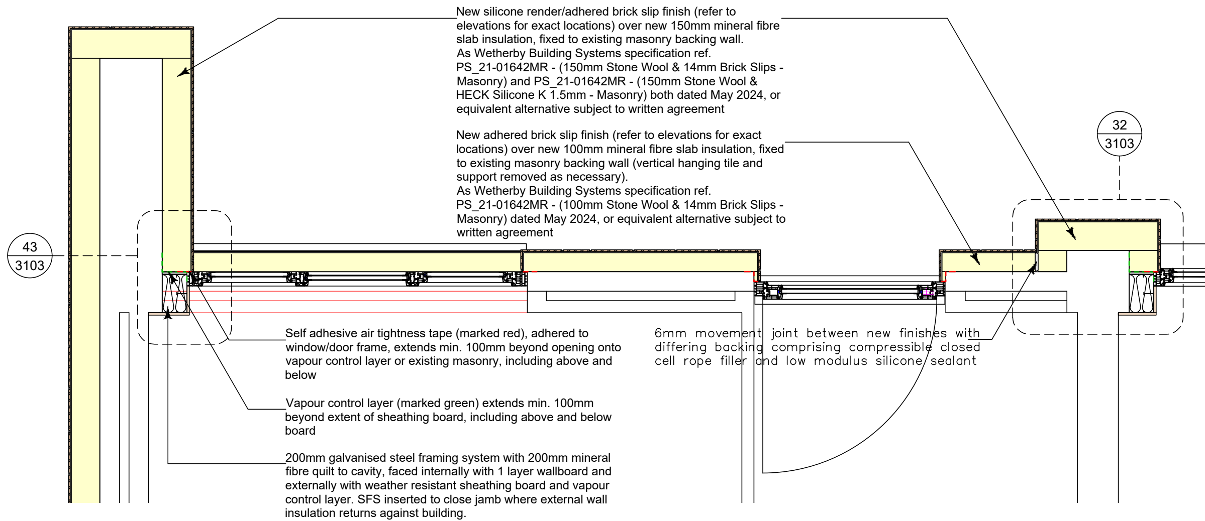
DETAIL 4 - GROUND FLOOR MAISONETTE REAR DOOR ENTRANCE
