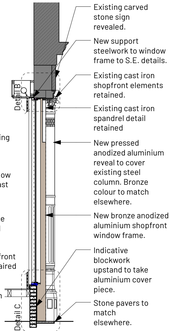
3 Proposed Shop Front Section Scale: 1:50
