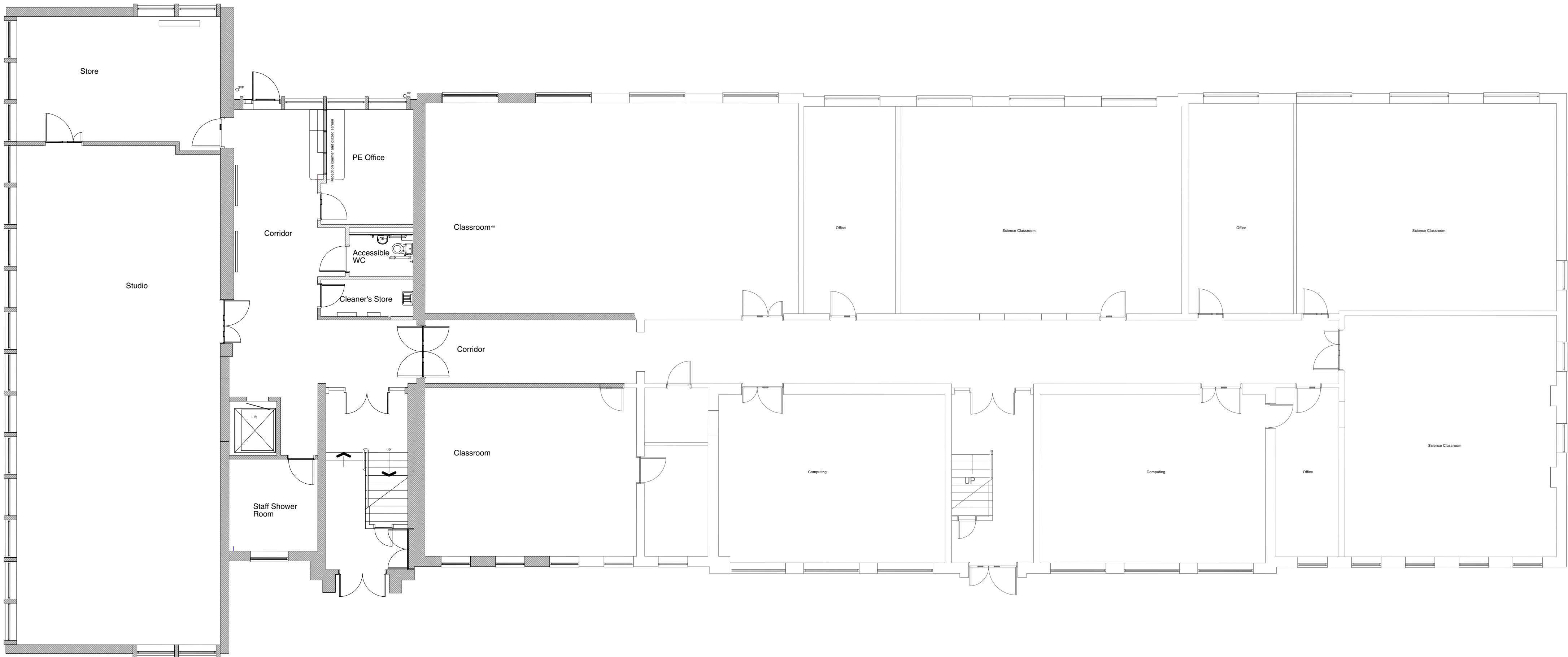
Ground Floor Existing Plan Science Building Scale: 1:100
