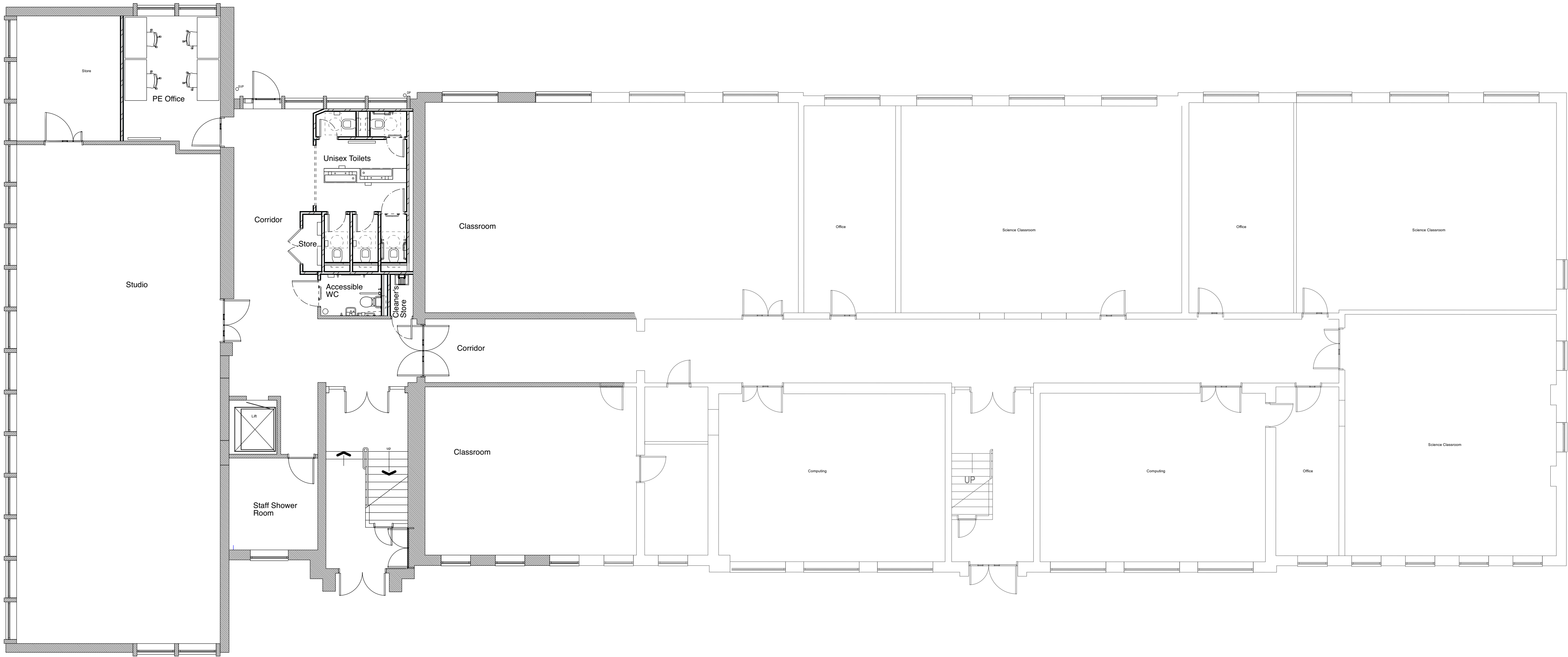
Ground Floor Proposed Plan Science Building Scale: 1:100
