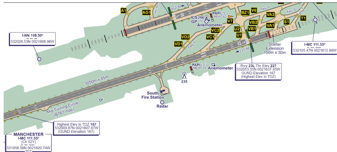
Figure 4 - Location of the SSR Site at Manchester Airport
