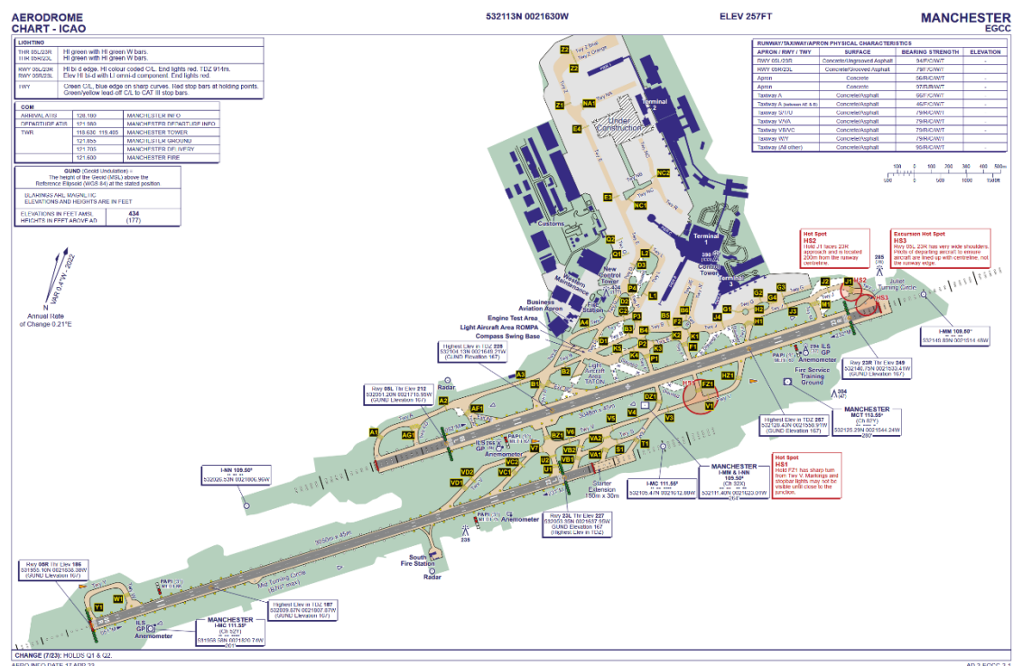
Figure 7 - Layout of Manchester Airport
