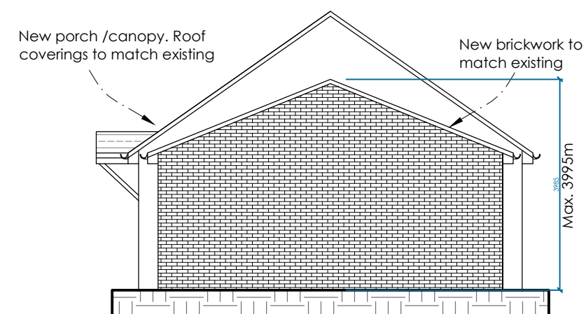
Side Elevation 1:100
