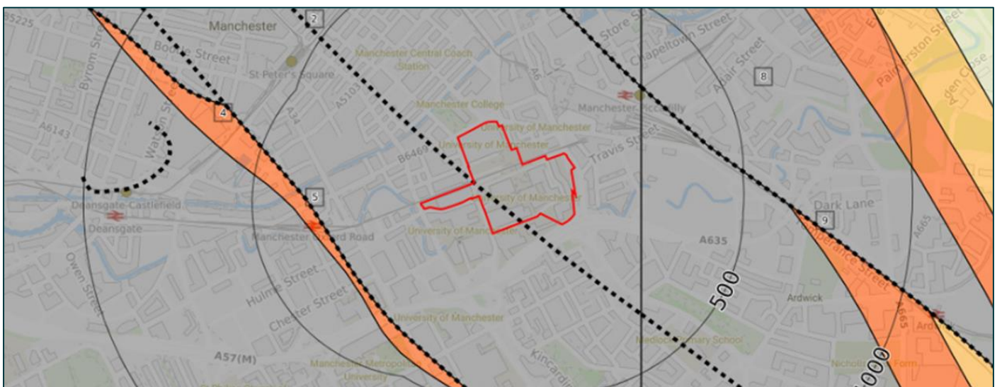
Plate 10: Bedrock Geology (based on excerpt from Groundsure Enviro + Geo Insight Report)
