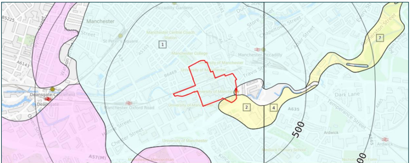
Plate 10: Bedrock Geology (based on excerpt from Groundsure Enviro + Geo Insight Report)
