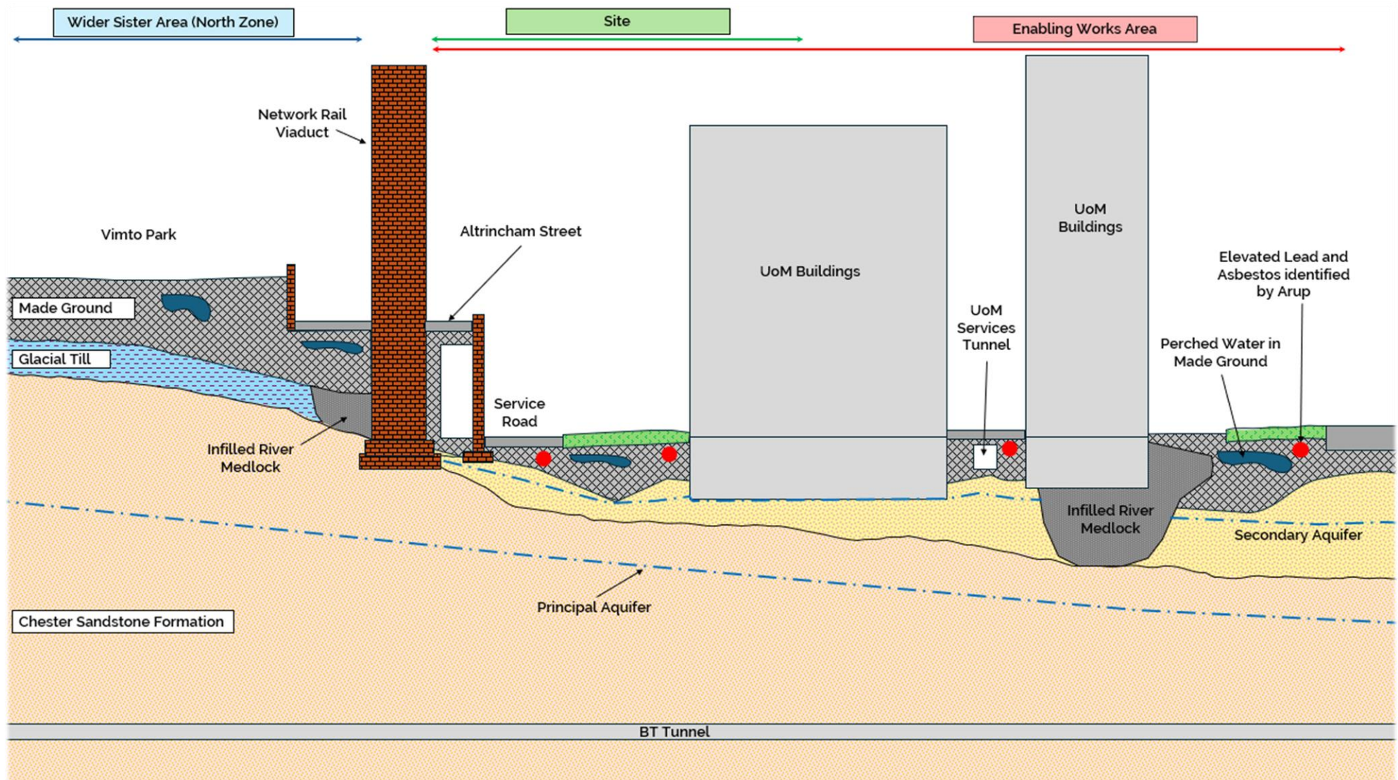
Plate 16: Illustrative Ground Model Cross Section (Northwest to Southeast, Not to Scale)
