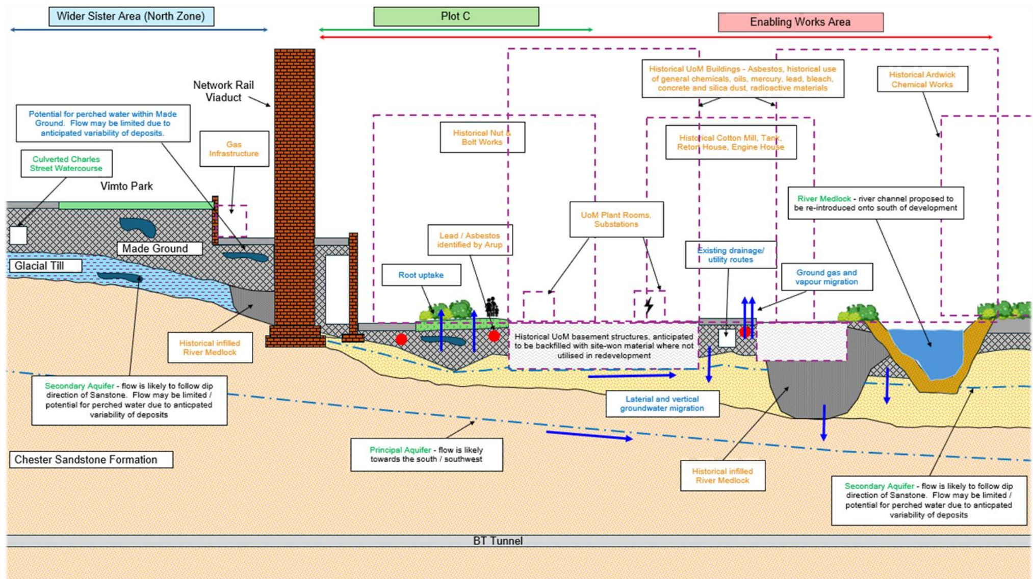
Plate 17. Illustrative Conceptual Site Model
