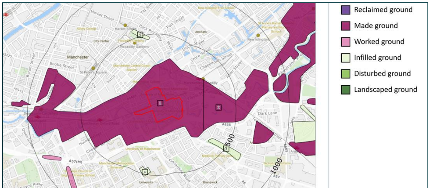
Plate 11: Excerpt from Groundsure Enviro + Geo Insight Report illustrated Worked Ground / Made Ground
