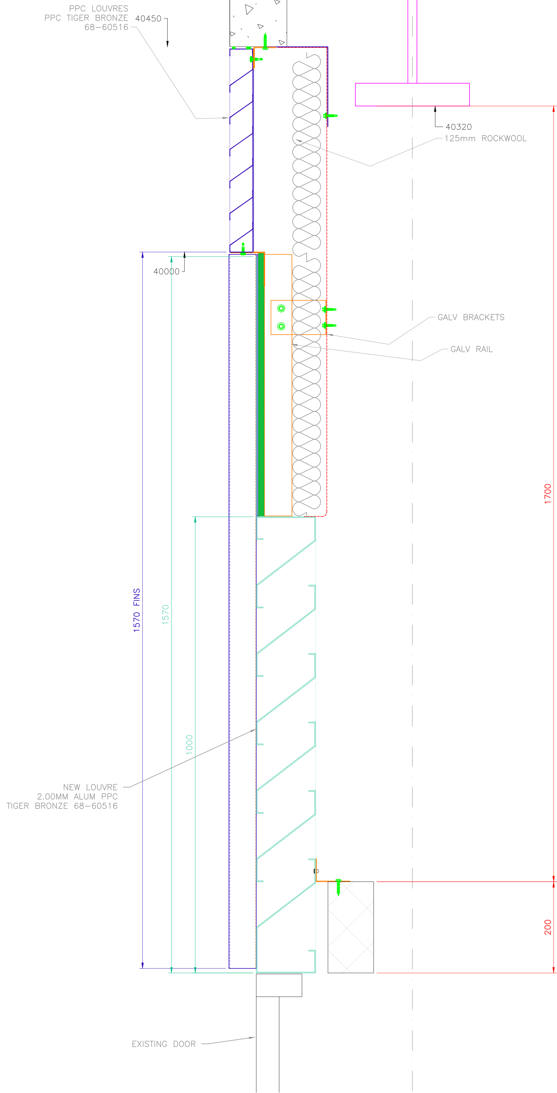
Typical Section - New Louvre Opening
