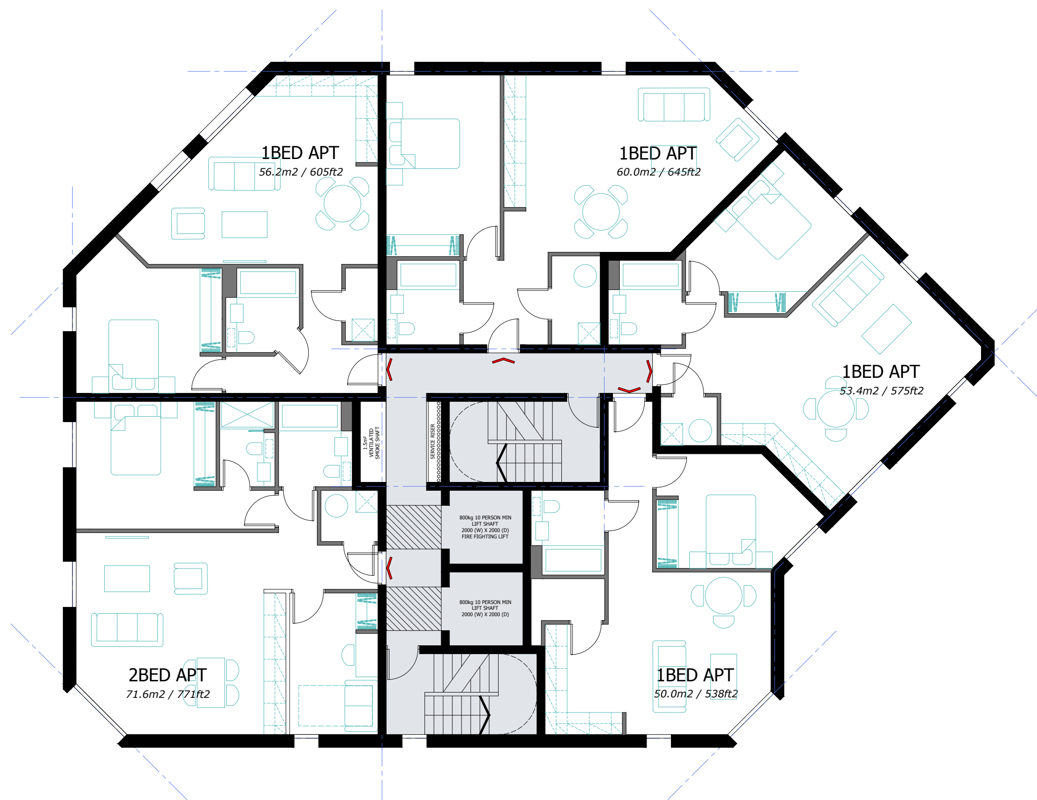
P Floors 3 - 5 as Proposed 1:100 @ A1
