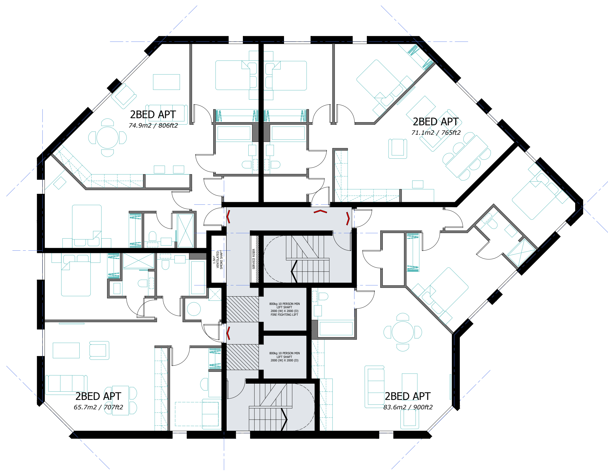
P Floors 6 - 11 as Proposed 1:100 @ A1
