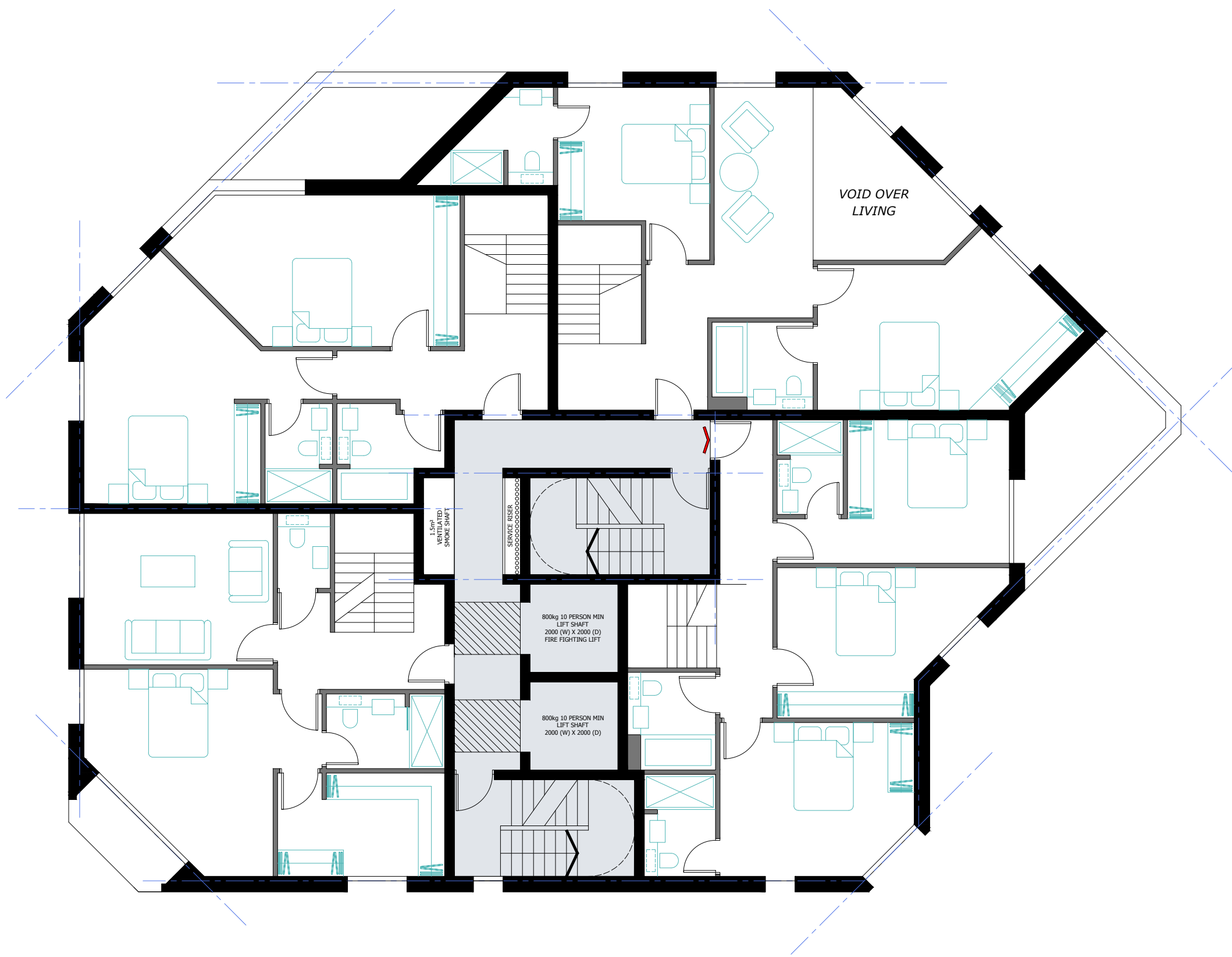
P Floor 14 as Proposed 1:100 @ A1
