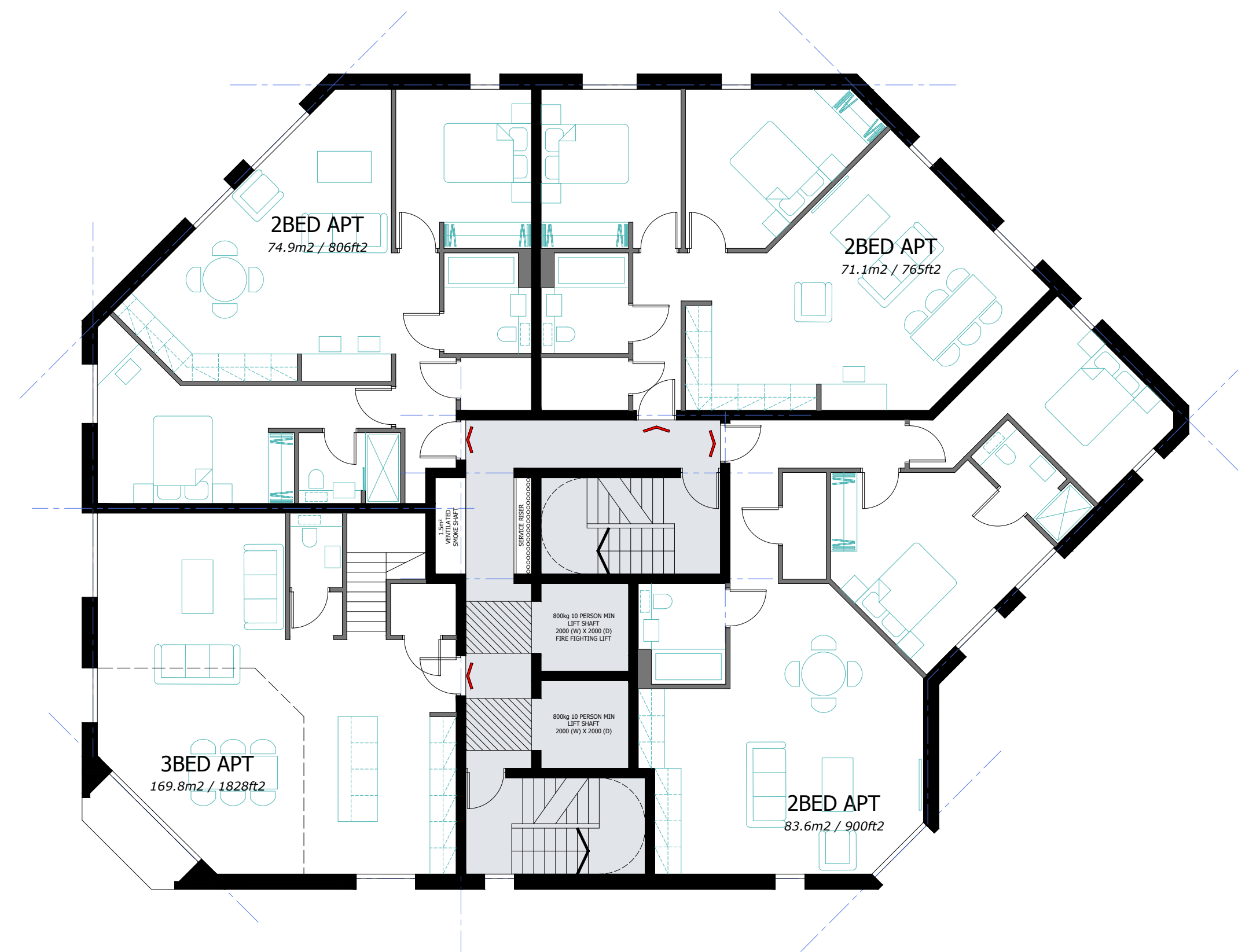
P Floor 12 as Proposed 1:100 @ A1
