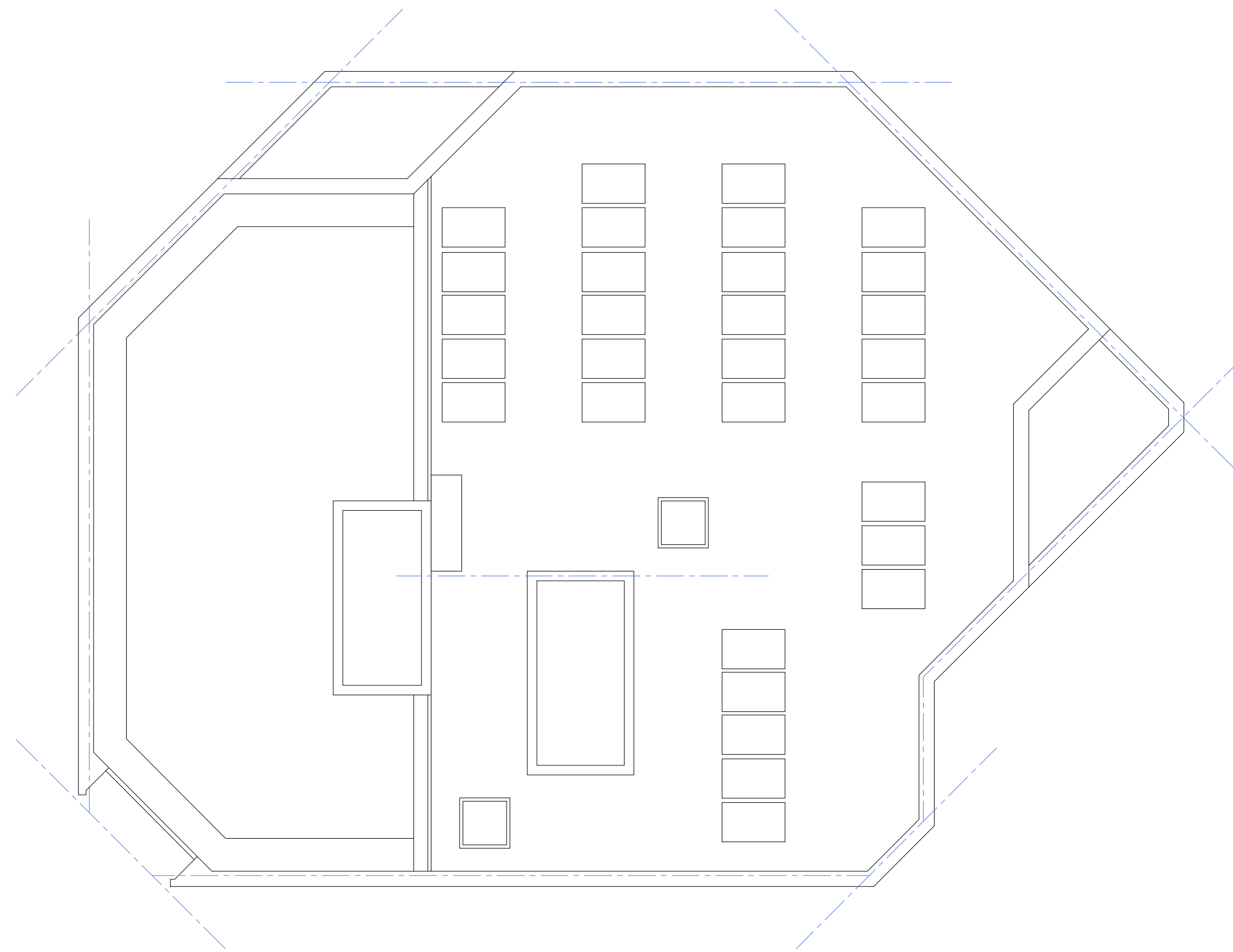
P Roof Plan as Proposed 1:100 @ A1
