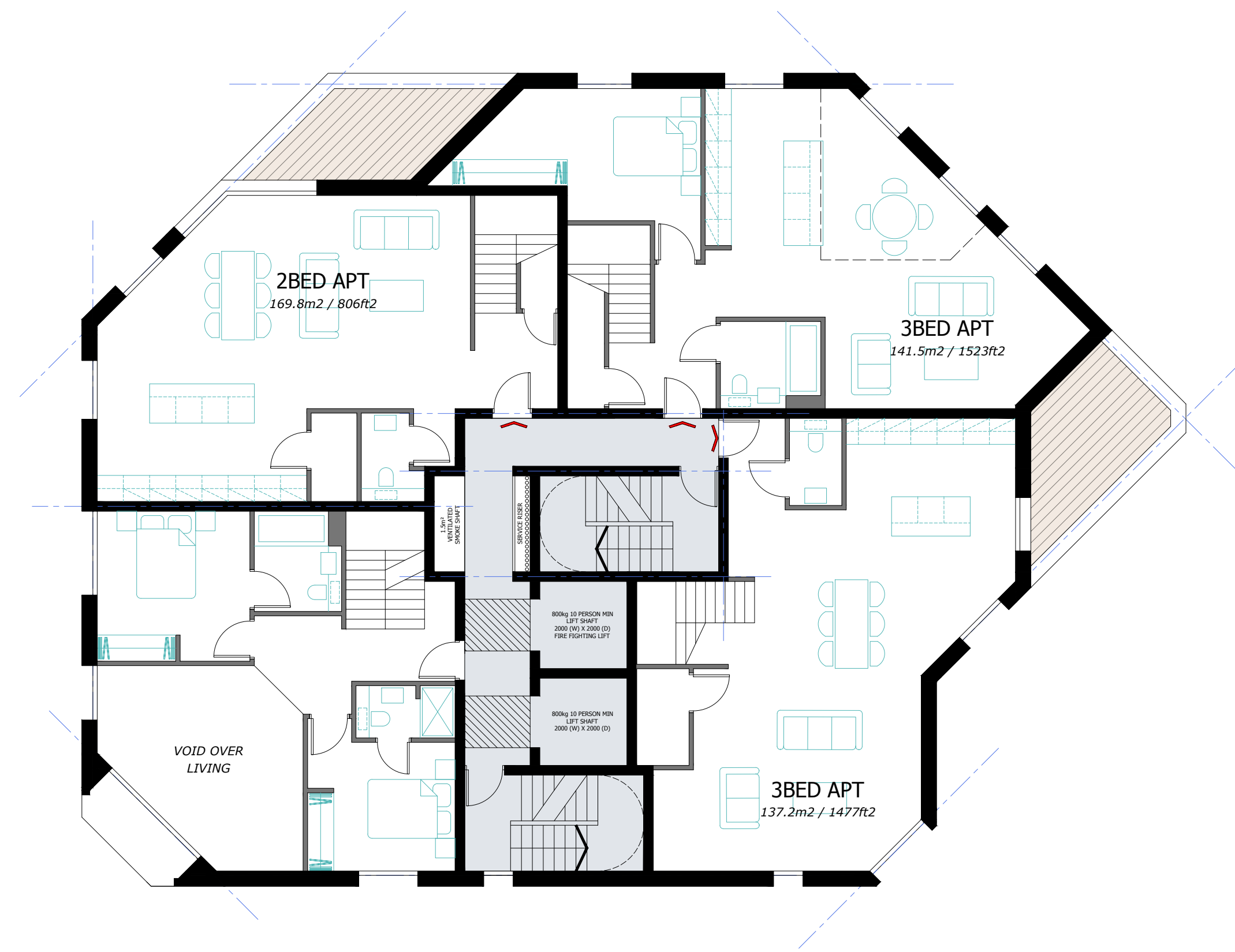
P Floor 13 as Proposed 1:100 @ A1
