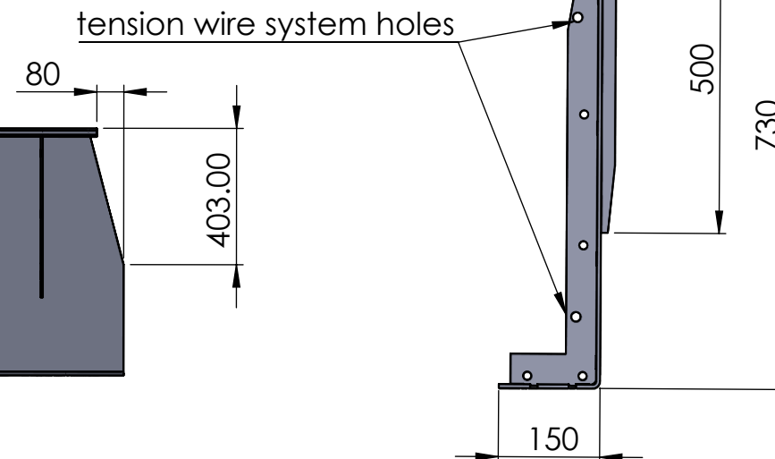
DETAIL E SCALE 1 : 20
