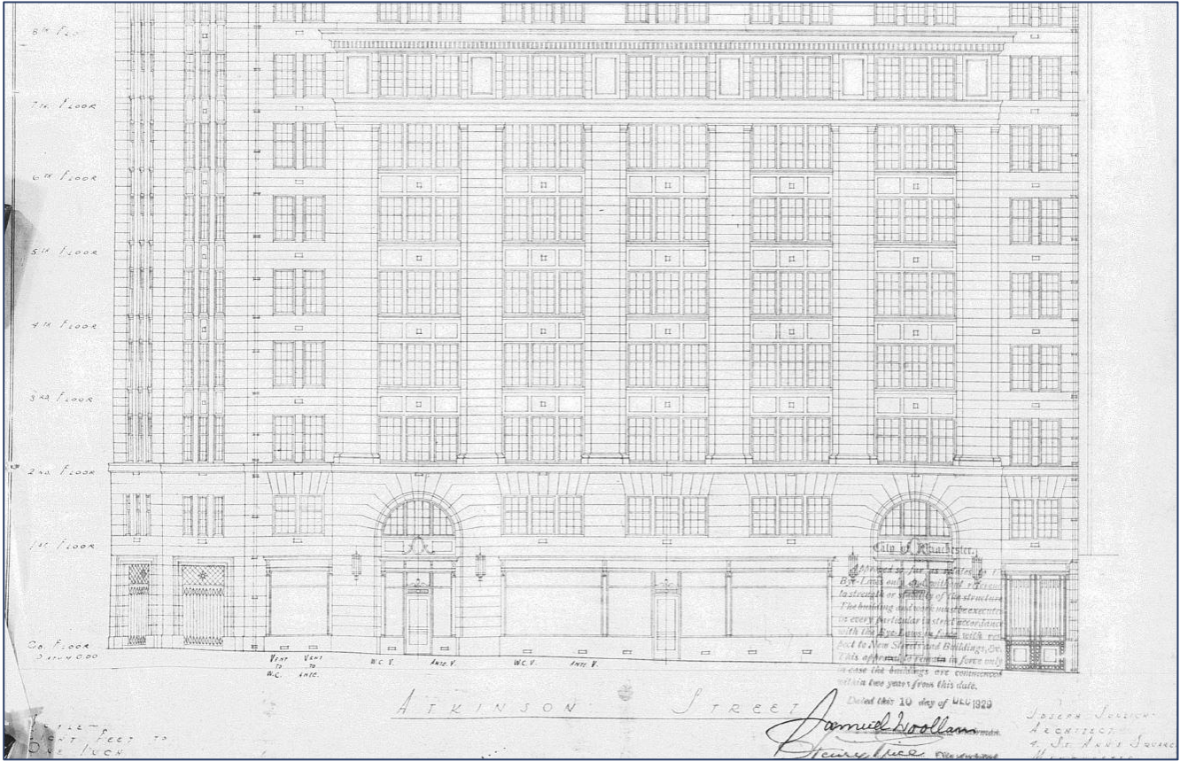
Image G – Atkinson Street elevation (1929)
