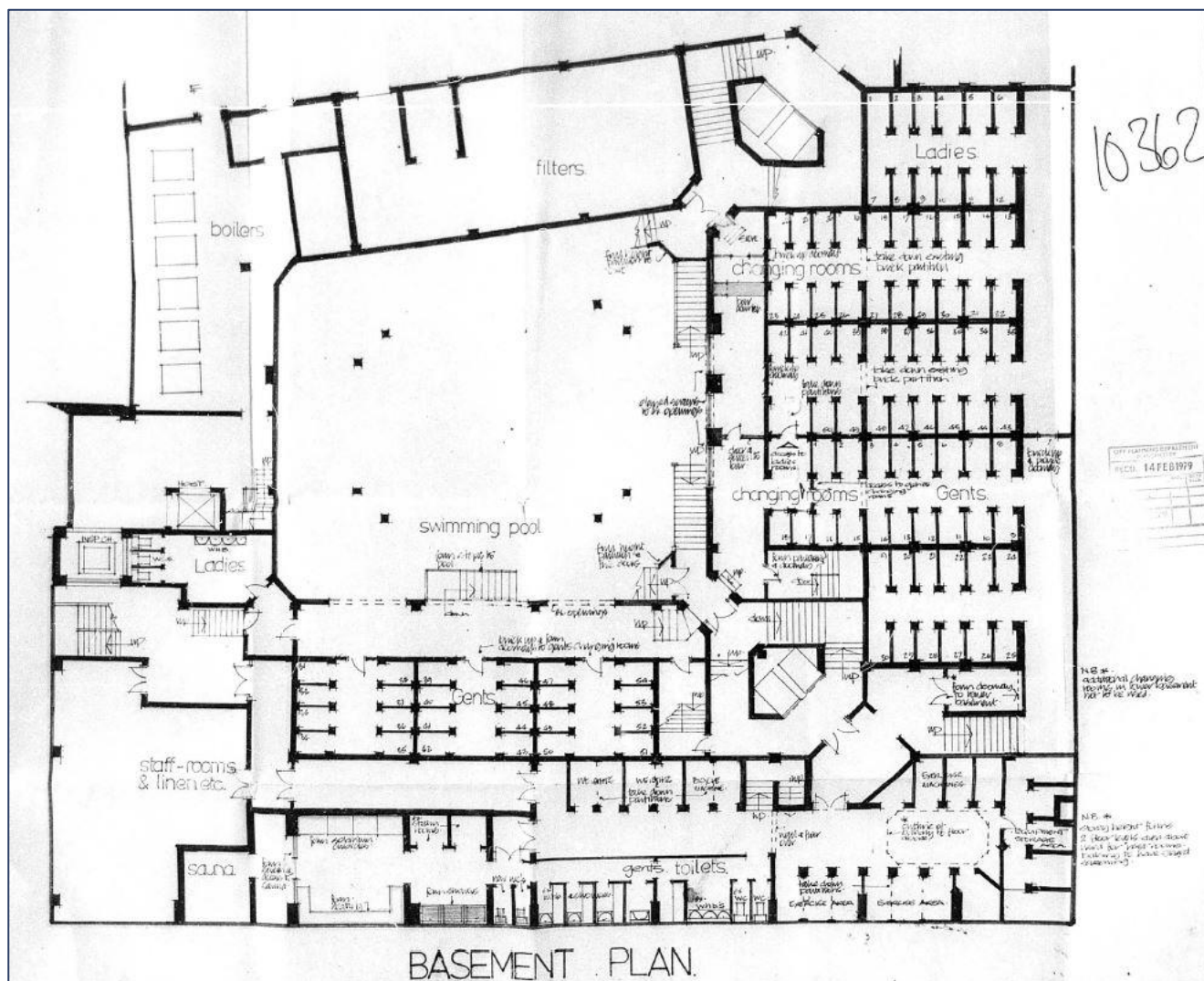
Figure 13 - Proposed basement plan submitted as part of the 1979 consented application (planning application reference: F10362)
