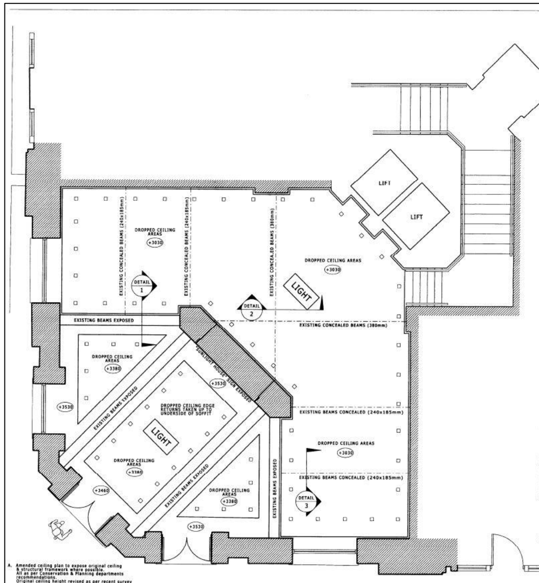
Figure 22 - Proposed changes to reception submitted as part of the 2008 application (085698/LO/2008/C1).
