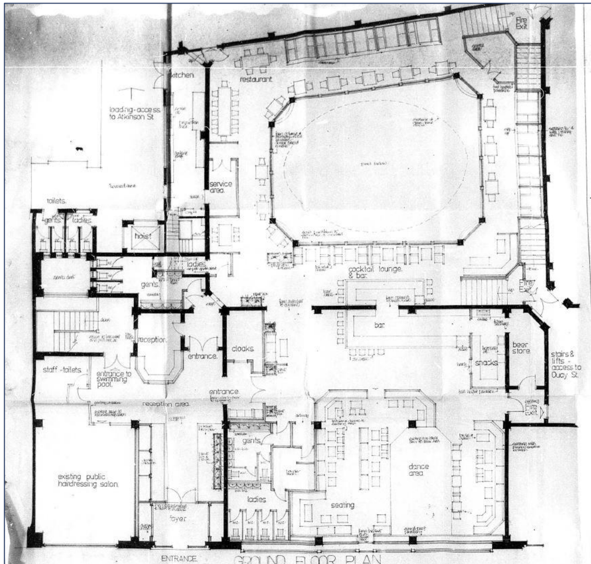
Figure 14 - Proposed ground floor plan submitted as part of the 1979 consented application (planning application reference: F10362)
