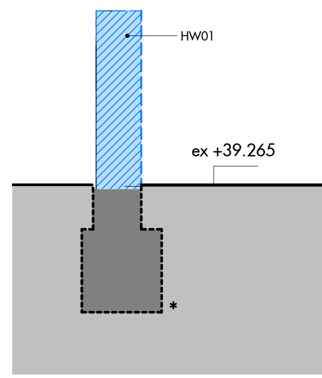
08 Holloway Wall Fabric Alterations Section AA 1 : 100
