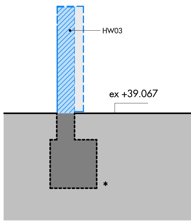
9 Holloway Wall Fabric Alterations Section BB 1 : 100
