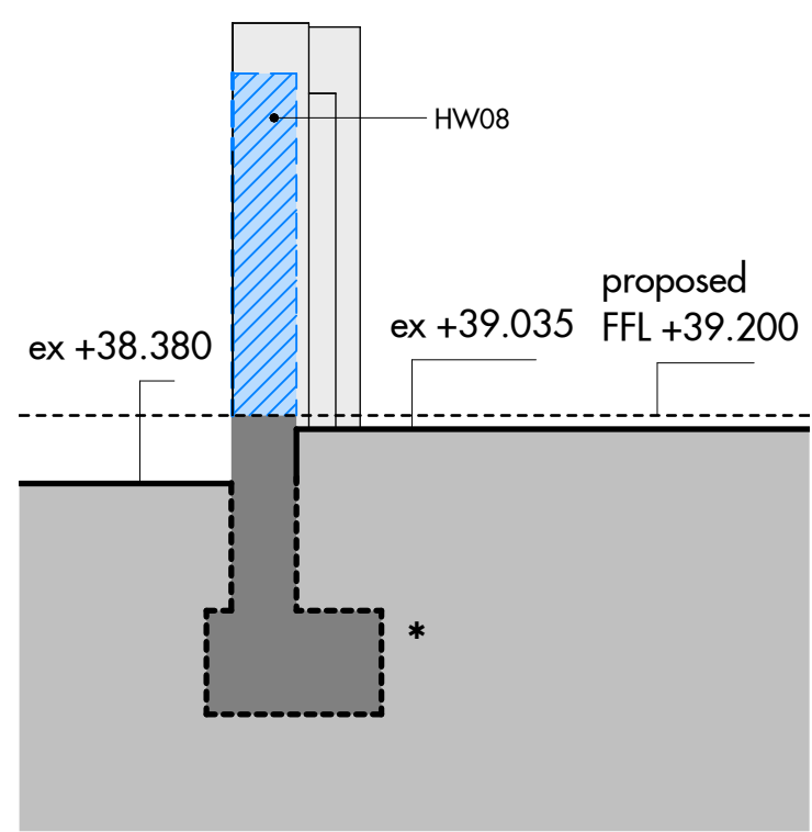
10 Holloway Wall Fabric Alterations Section CC 1 : 100
