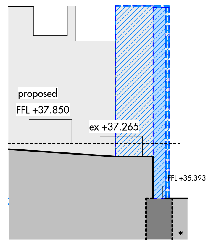
12 Holloway Wall Fabric Alterations Section EE 1 : 100
