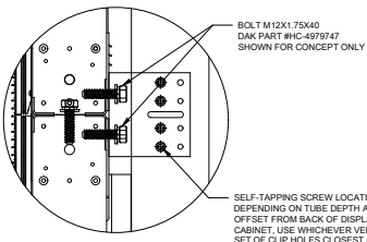
DETAIL D SCALE 1:10
