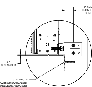
DETAIL C SCALE 1:10
