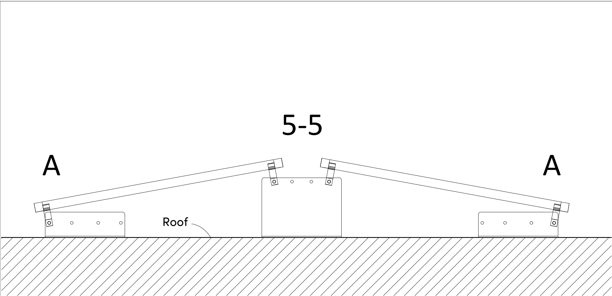
E/W System With Universal Supports For Low Ballast Requirements
