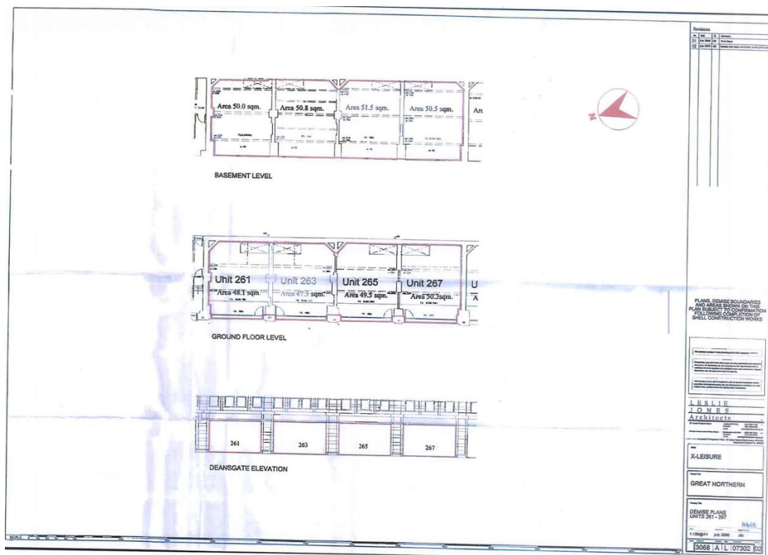
Demise Plans: July 2008, Stair to rear RH corner of unit 265
