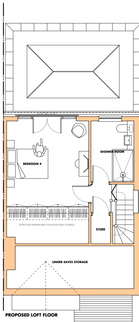
PROPOSED LOFT FLOOR
