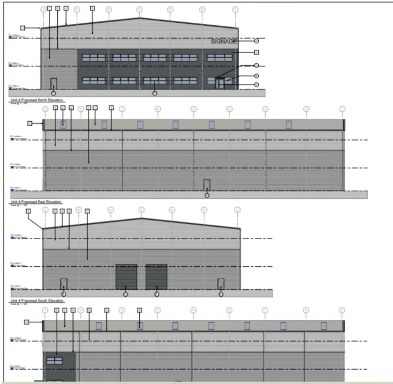
Unit 4 – previously approved elevations
