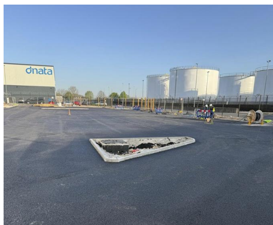
Install of porous top course
