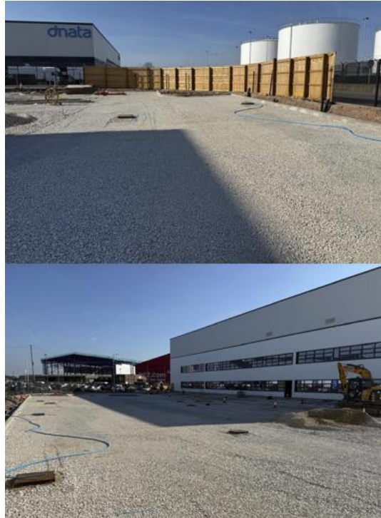
Install of type 3 sub-base
