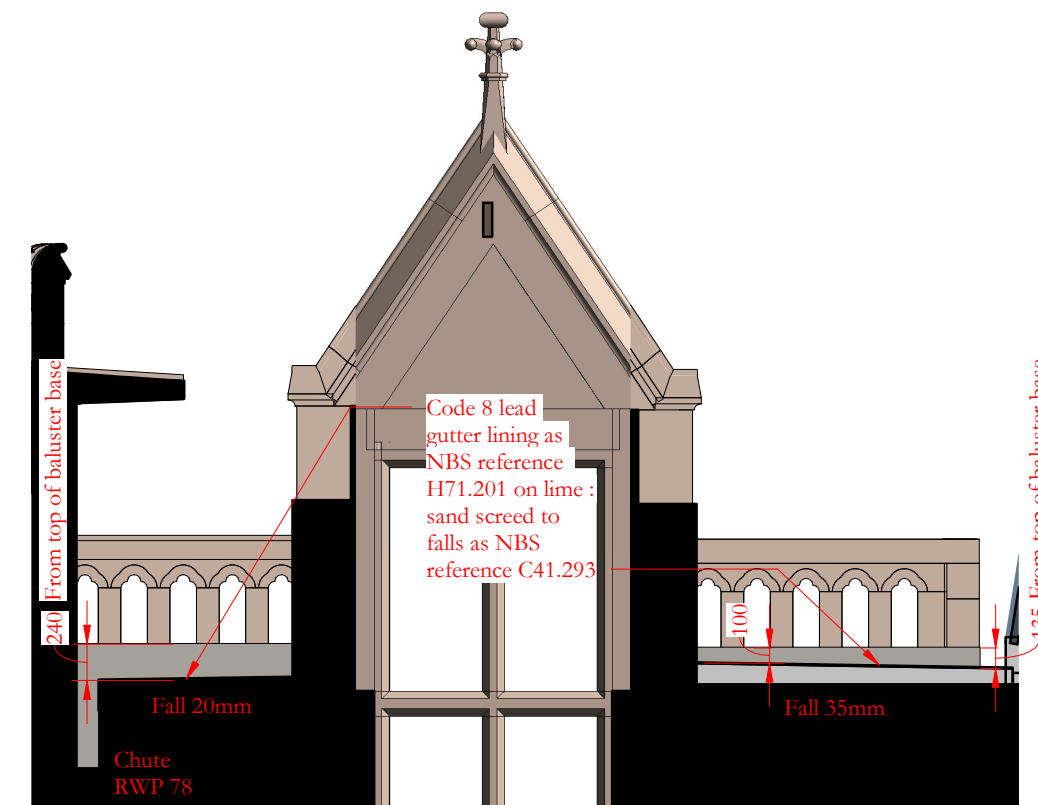
Princess Street courtyard east gutter roof slope CBR01
