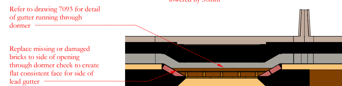
Gutter through dormer SCR02b2
