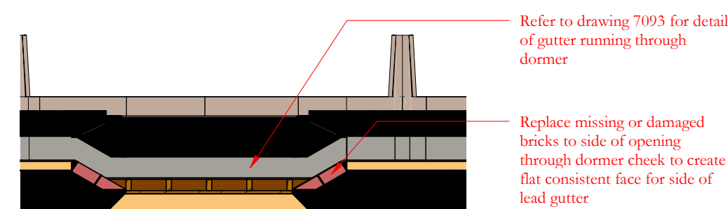
Gutter through dormer NCR03d2
