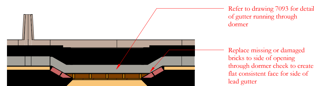
Gutter through dormer NCR03d4
