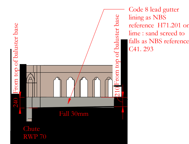
Princess Street courtyard north-west gutter roof slope NCR03b
