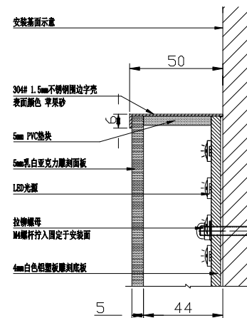
侧剖图 Side Section View
