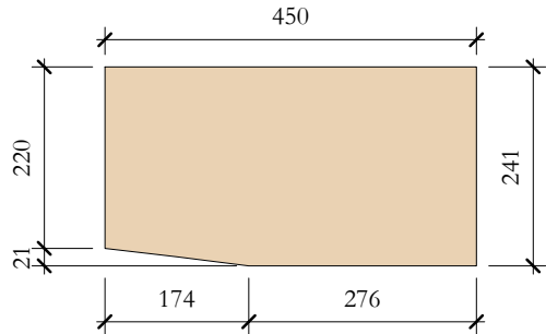
TcR_35 Elevation Front 1 : 10
