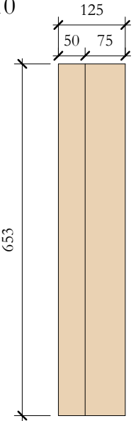
TcW_05 Elevation Left 1 : 10
