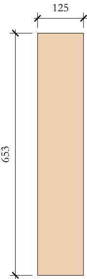
TcW_06 Elevation Left 1 : 10
