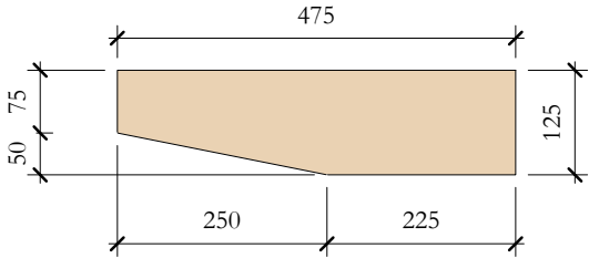
TcW_06 Elevation Top 1 : 10
