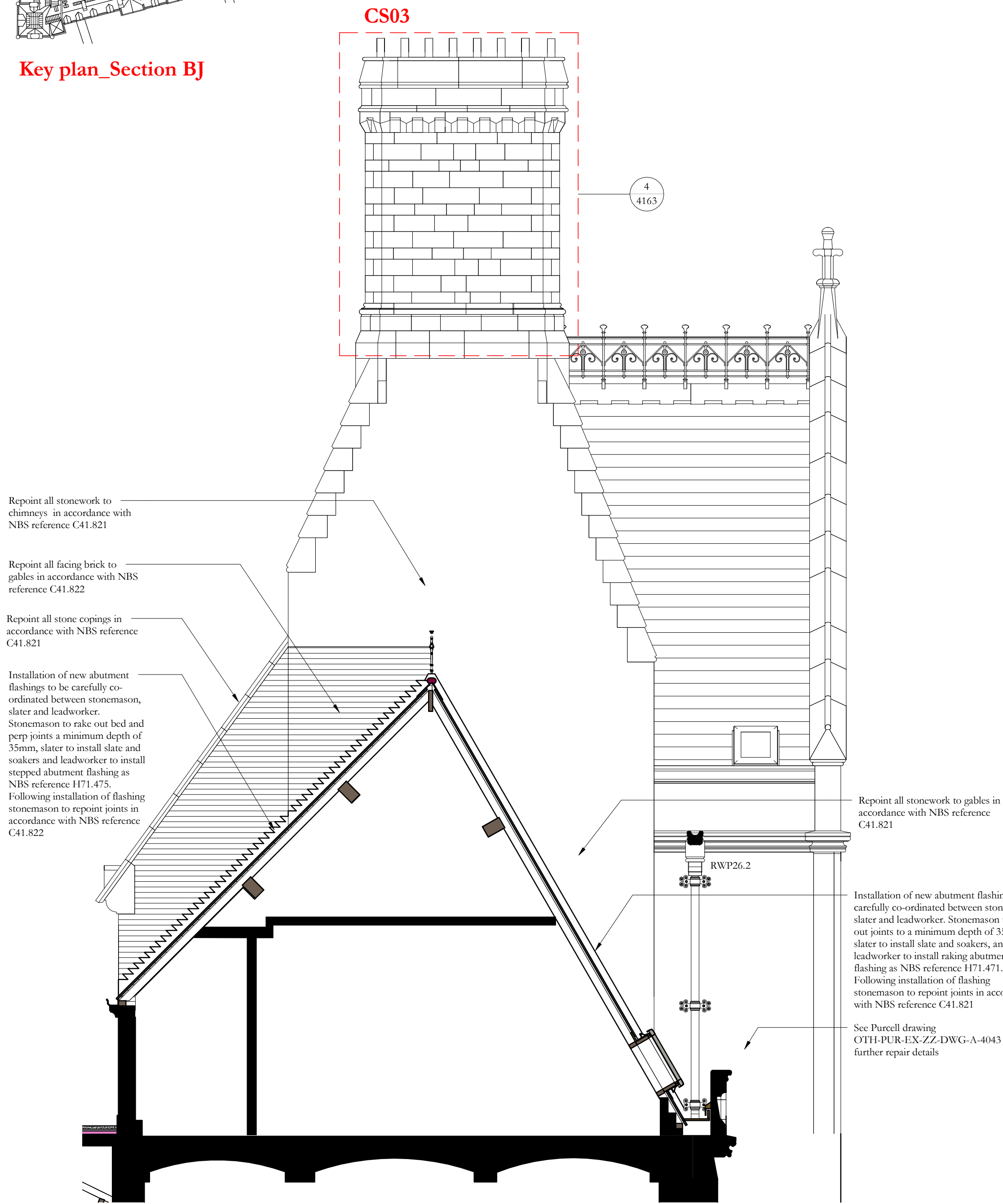
Section BJ
