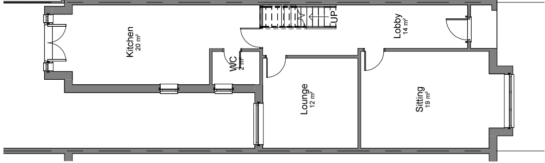
00-E-Ground Floor 1 : 100
