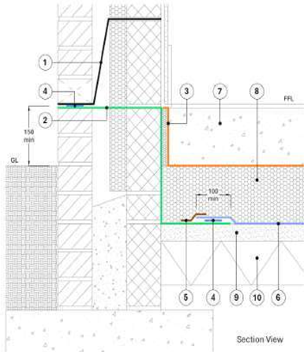
Diagram 2 - Typical detail below slab and insulation
