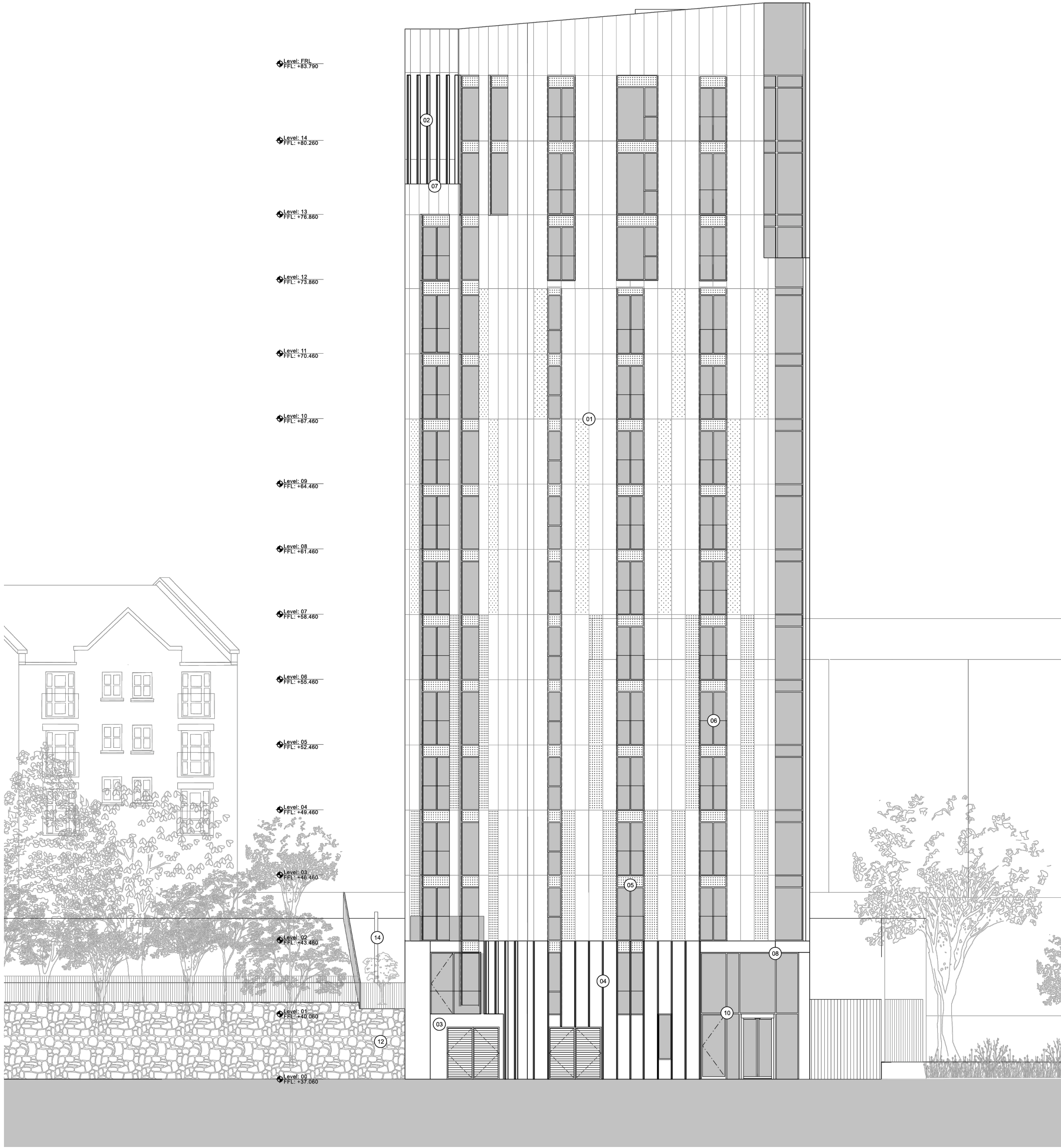
E Store St Elevation as Approved 1:100 @ A1
