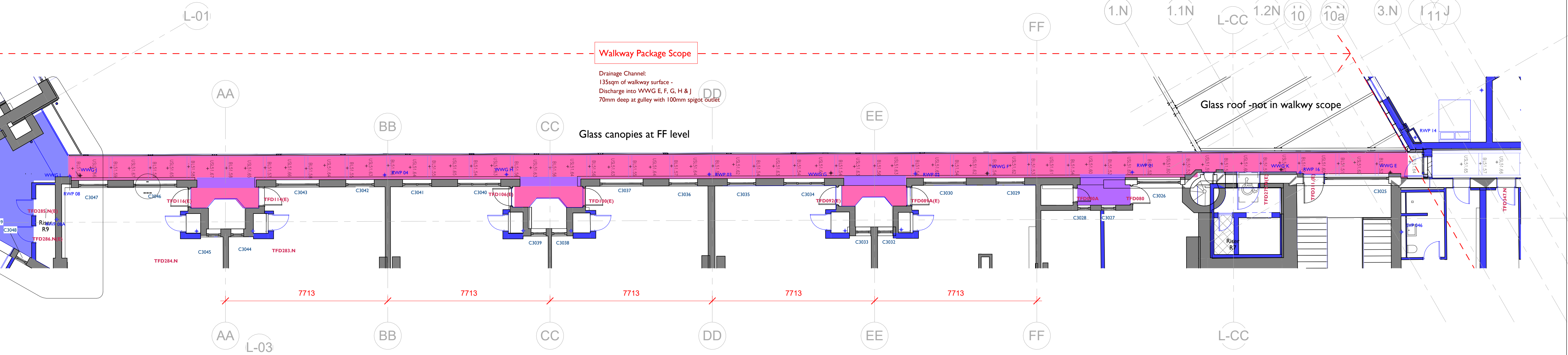
1 03 Third Floor - Fairfield St Walkway 4112 I : 100
