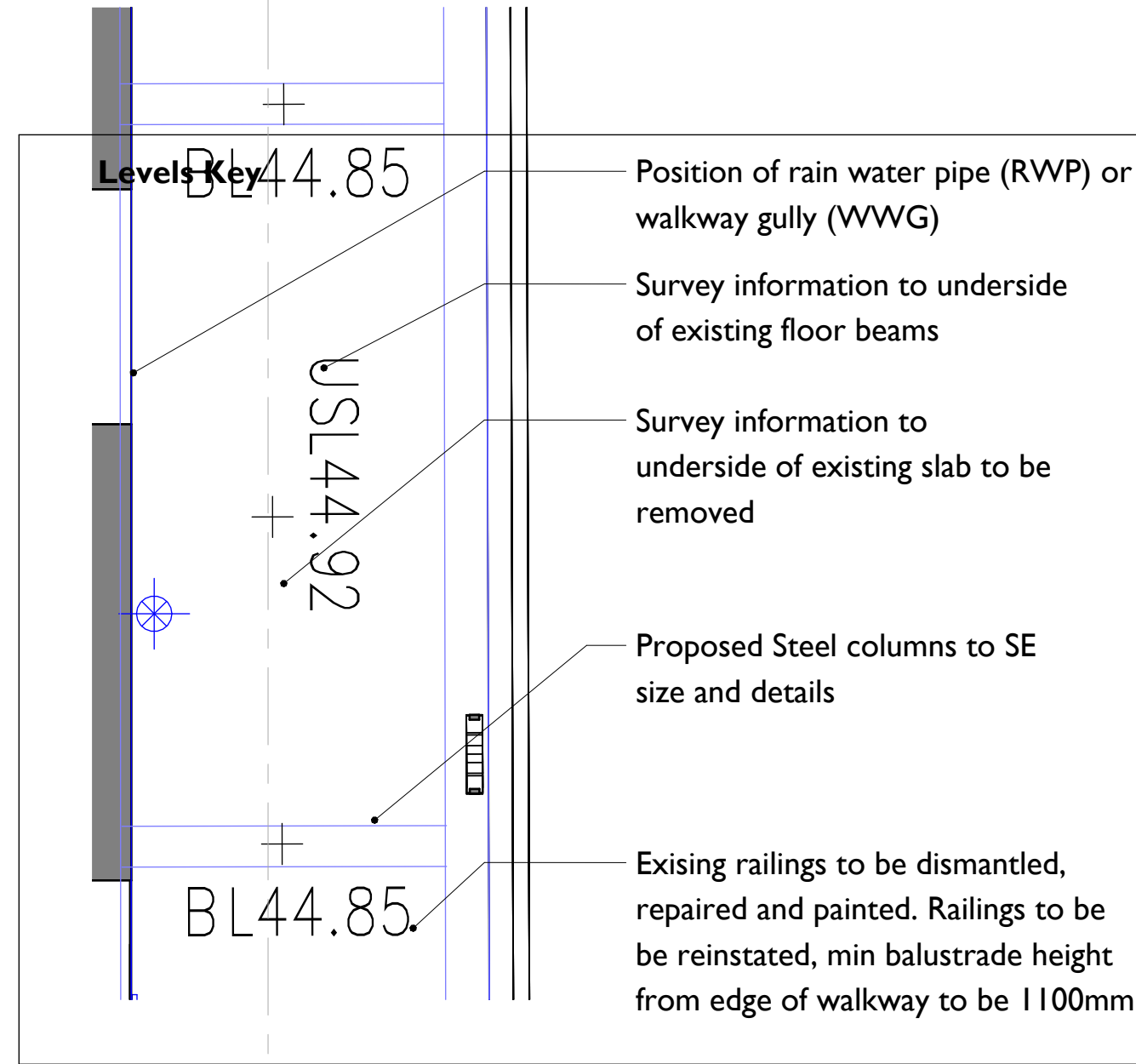
1 03 Third Floor - Fairfield St Walkway 4112 I : 100
