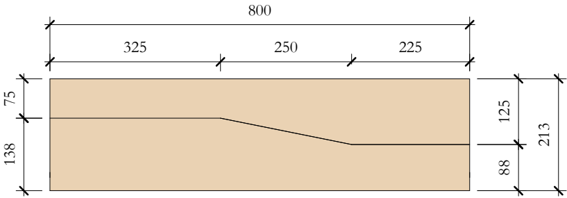
TcS_05 Elevation Top
