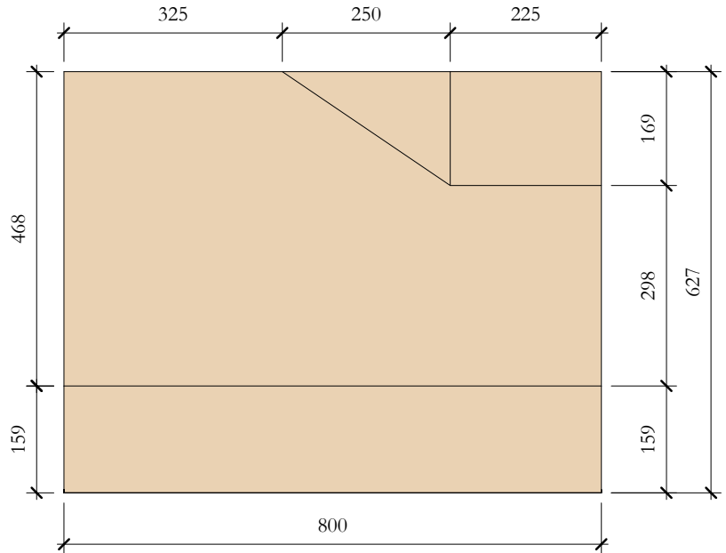
TcS_05 Elevation Front
