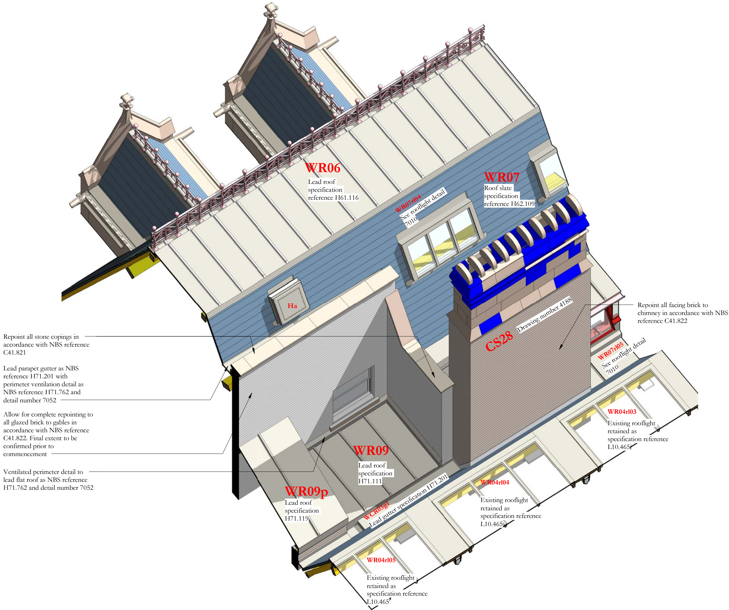
Key plan_West Roof 3D 1 : 1250
