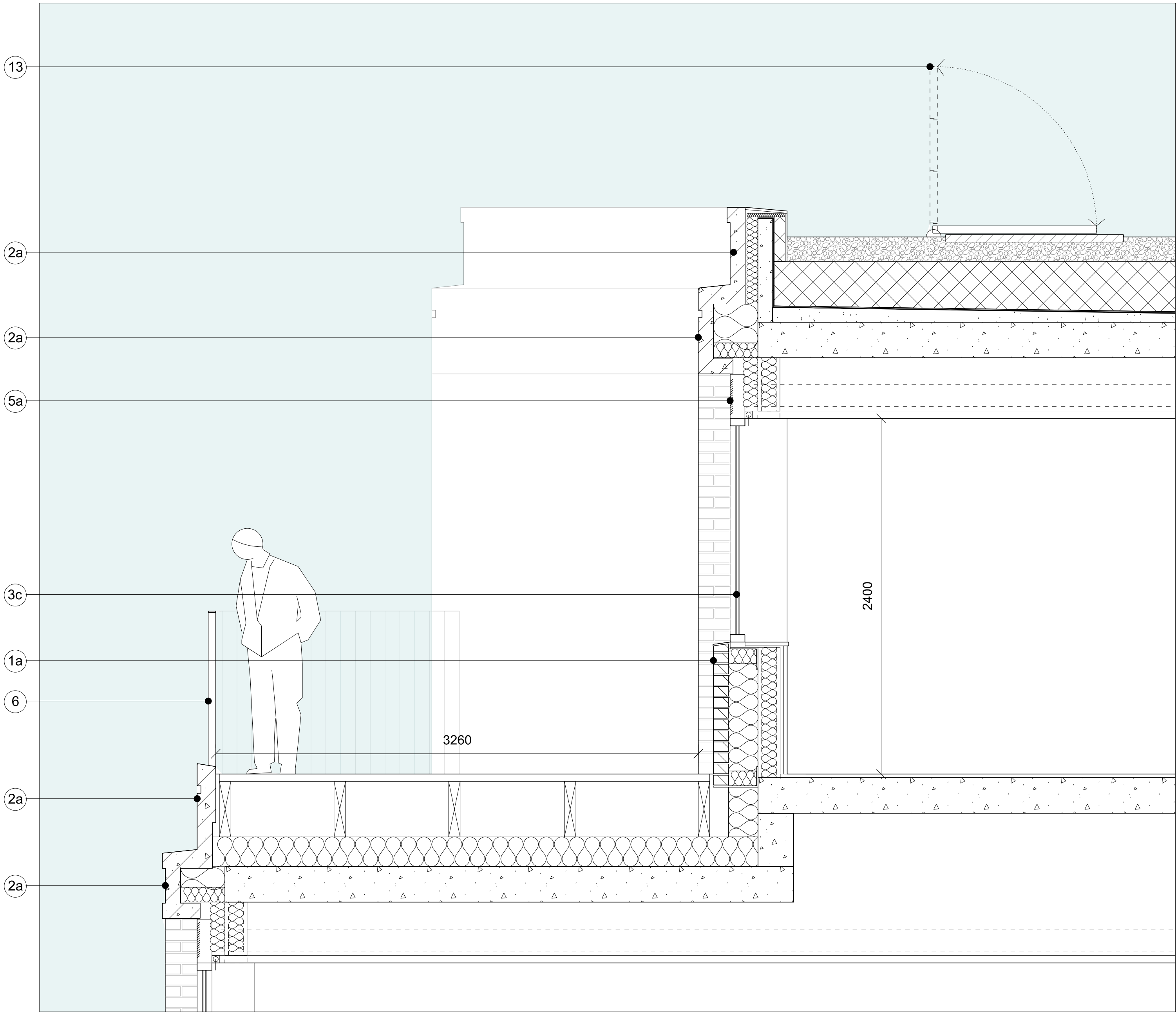
01 Section AA 1:20 @ A1
