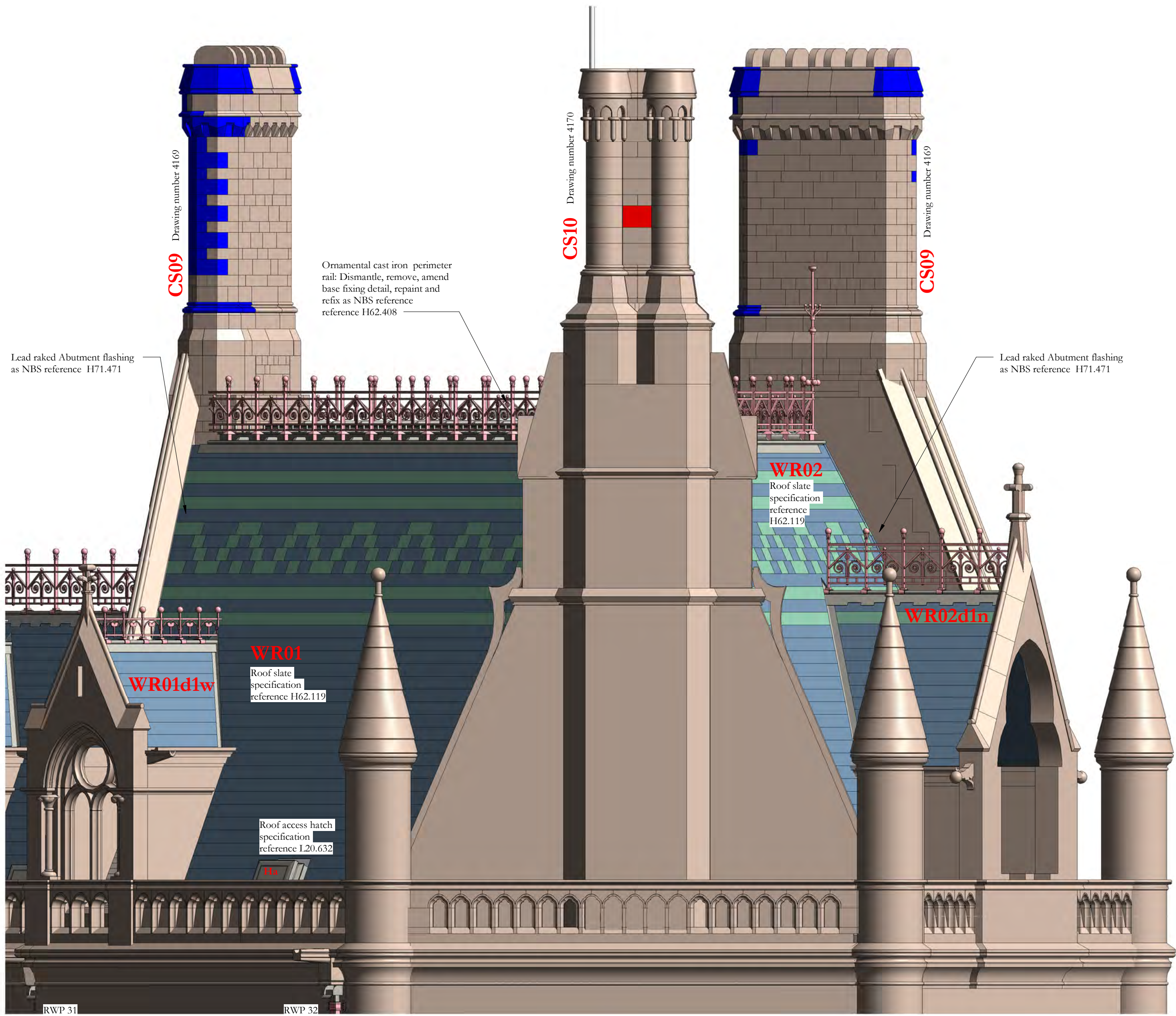
Princess Street and Albert Square corner roof elevation 1 : 50
