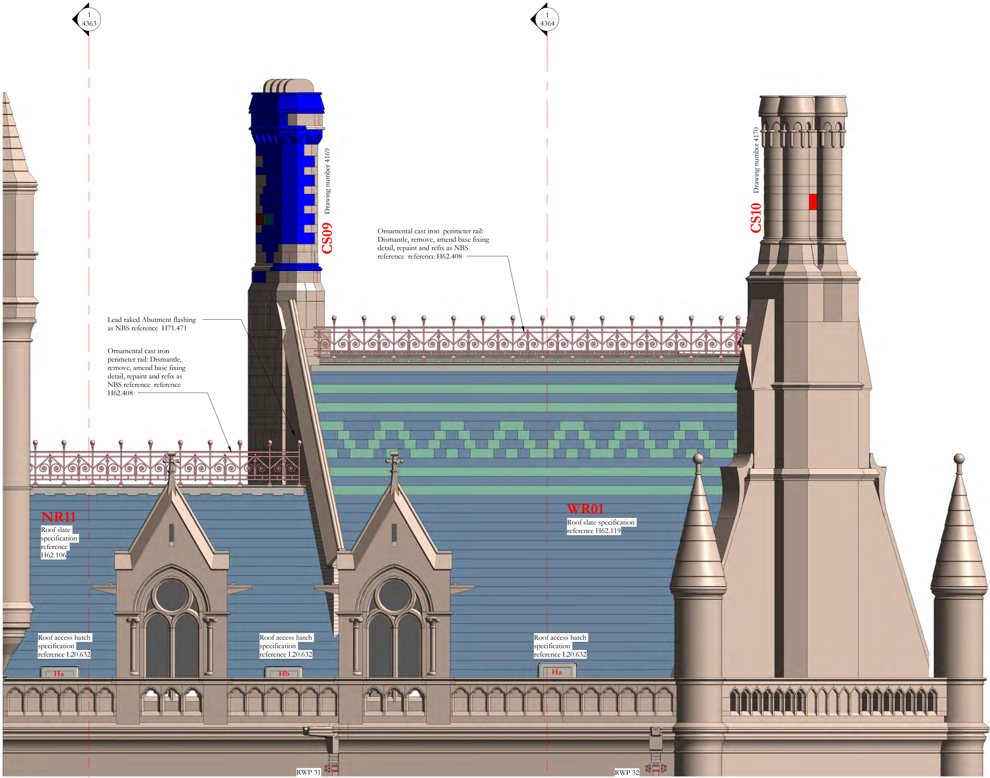
Princess Street roof elevation 6 1 : 50
