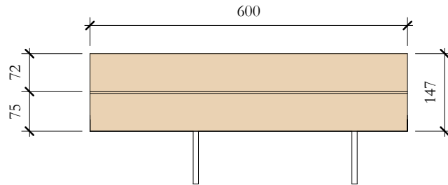
TcC_13 Elevation Front 1 : 10
