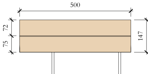
TcC_14 Elevation Front 1 : 10
