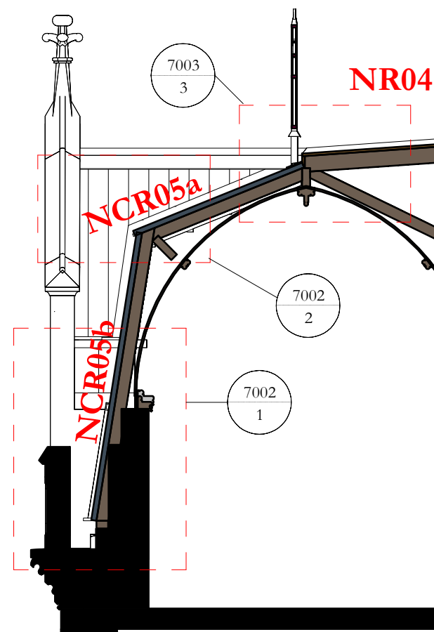
Section LL 1 : 50
